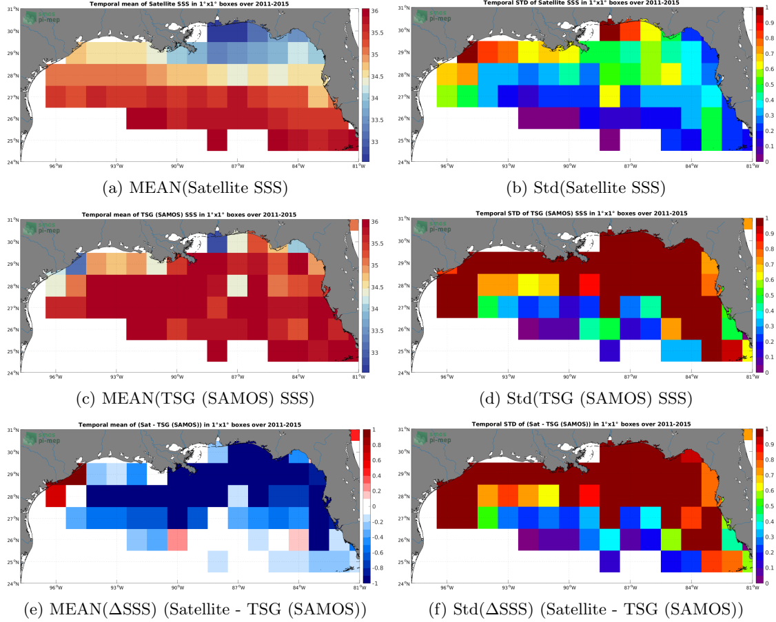
Figure 6: Temporal mean (left) and Std (right) of SSS from Aquarius SSS L4 OI v5 - Monthly (IPRC) (top), TSG (SAMOS) (middle), and of \Delta\text{SSS} (Satellite - TSG (SAMOS)). Only match-up pairs are used to generate these maps.
