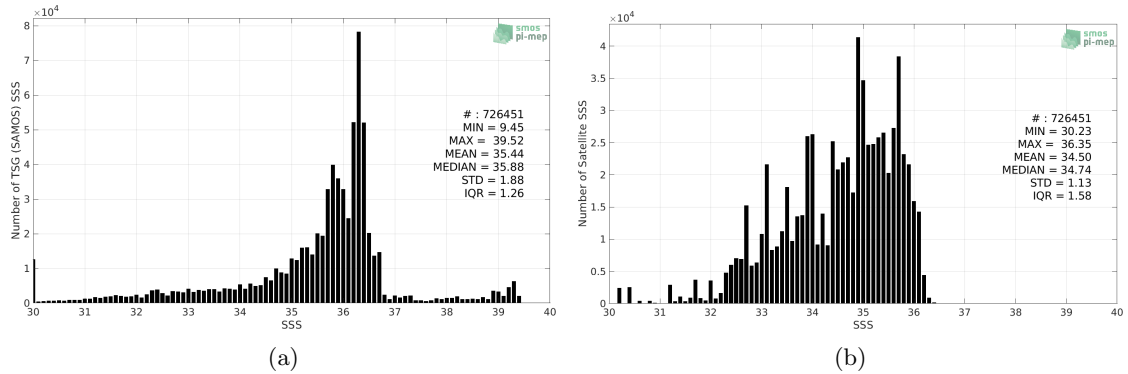
Figure 2: Histograms of SSS from TSG (SAMOS) (a) and Aquarius SSS L4 OI v5 - Monthly (IPRC) (b) considering all match-up pairs per bins of 0.1 over the Mississippi river plume Pi-MEP region and for the full satellite product period.
