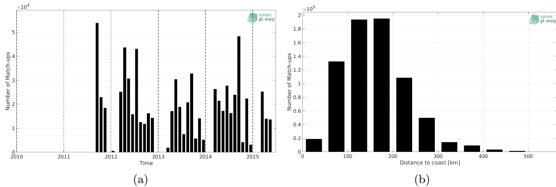
Figure 1: Number of match-ups between TSG (SAMOS) and Aquarius SSS L4 OI v5 - Monthly (IPRC) SSS as a function of time (a) and as function of the distance to coast (b) over the Mississippi river plume Pi-MEP region and for the full satellite product period.
