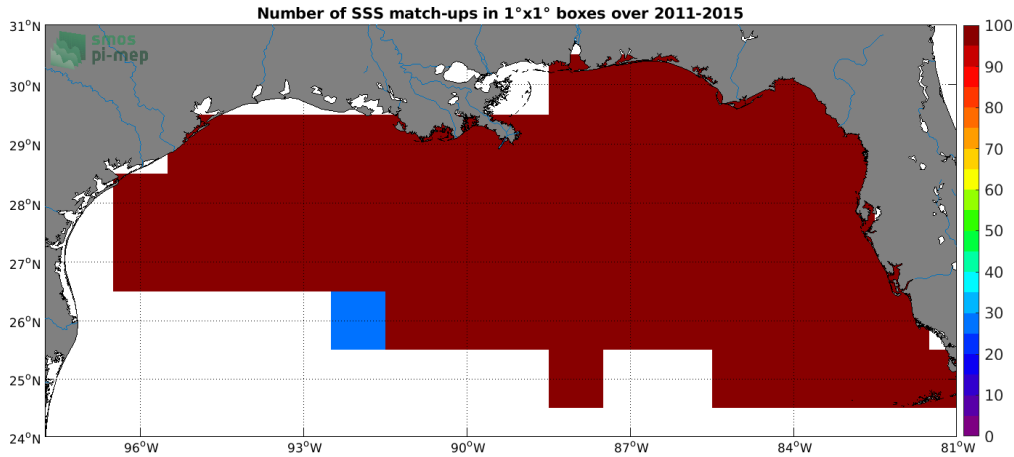
Figure 4: Number of SSS match-ups between TSG (SAMOS) SSS and the Aquarius SSS L4 OI v5 - Monthly (IPRC) SSS product for the Mississippi river plume Pi-MEP region over 1^\circ \times 1^\circ boxes and for the full satellite product period.
