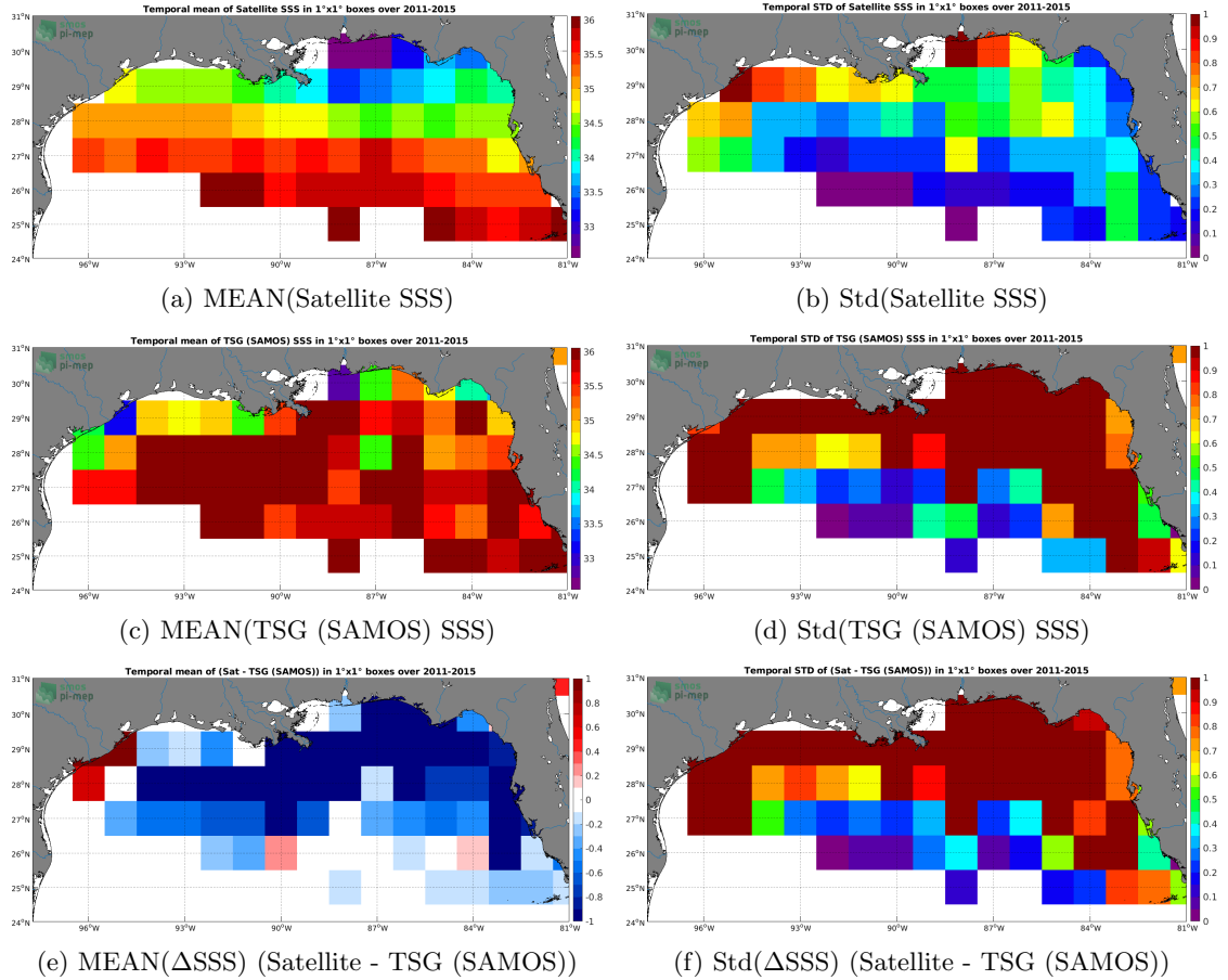
Figure 6: Temporal mean (left) and Std (right) of SSS from Aquarius SSS L4 OI v5 - Monthly (IPRC) (top), TSG (SAMOS) (middle), and of \Delta\text{SSS}(\text{Satellite} - \text{TSG}(\text{SAMOS})) . Only match-up pairs are used to generate these maps.
