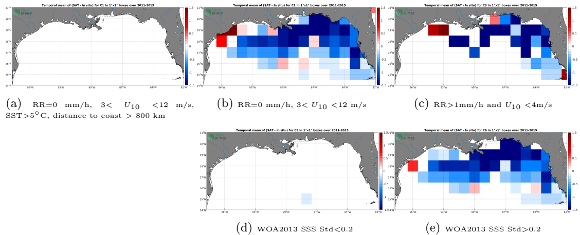
Figure 12: Temporal mean gridded over spatial boxes of size 1^{\circ}\times 1^{\circ} of \Delta\text{SSS} (Aquarius SSS L4 OI v5 - Monthly (IPRC) - TSG (SAMOS)) for 5 different subdatasets corresponding to:RR=0 mm/h, 3 < U_{10} < 12 m/s, SST > 5^{\circ}\text{C} , distance to coast > 800 km (a), RR=0 mm/h, 3 < U_{10} < 12 m/s (b), RR > 1 mm/h and U_{10} < 4 m/s (c), WOA2013 SSS Std < 0.2 (d), WOA2013 SSS Std > 0.2 (e).
