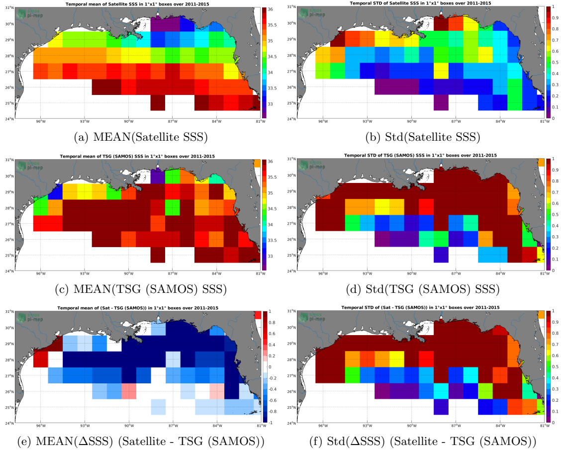
Figure 6: Temporal mean (left) and Std (right) of SSS from Aquarius SSS L4 OI v5 - Monthly (IPRC) (top), TSG (SAMOS) (middle), and of \Delta SSS (Satellite - TSG (SAMOS)). Only match-up pairs are used to generate these maps.
