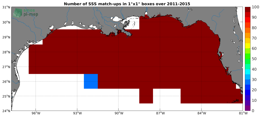
Figure 4: Number of SSS match-ups between TSG (SAMOS) SSS and the Aquarius SSS L4 OI v5 - Monthly (IPRC) SSS product for the Mississippi river plume Pi-MEP region over 1°x1° boxes and for the full satellite product period.
