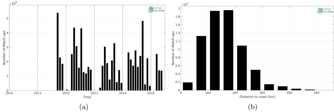
Figure 1: Number of match-ups between TSG-SAMOS and Aquarius-L4-IPRC-V5-MONTHLY SSS as a function of time (a) and as function of the distance to coast (b) over the Mississippi river plume Pi-MEP region and for the full satellite product period.
