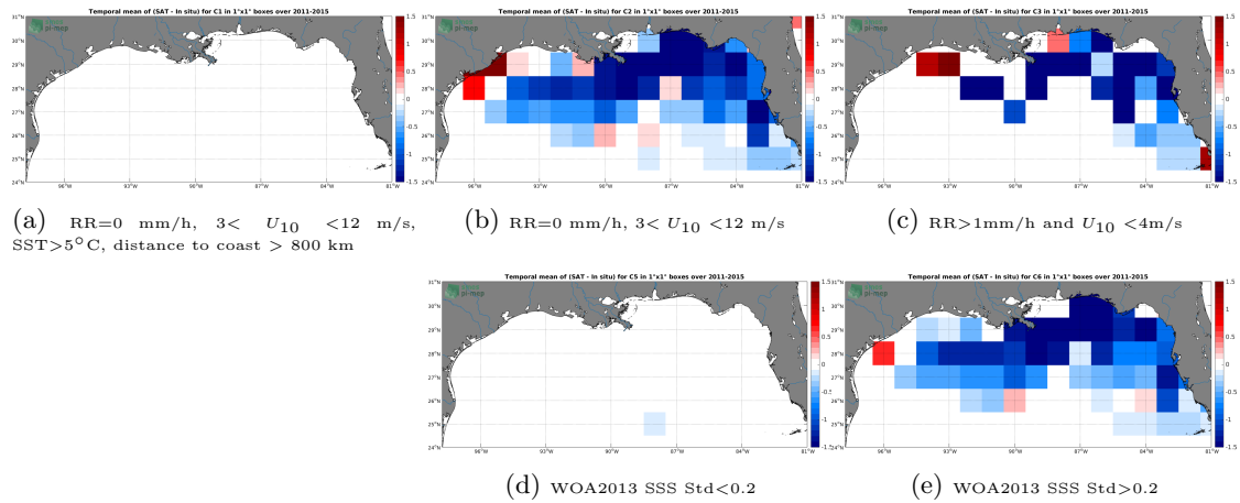
Figure 12: Temporal mean gridded over spatial boxes of size 1^{\circ}\times 1^{\circ} of \Delta\text{SSS} (Aquarius-L4-IPRC-V5-MONTHLY - TSG-SAMOS) for 5 different subdatasets corresponding to:RR=0 mm/h, 3 < U_{10} < 12 m/s, SST >5^{\circ}\text{C} , distance to coast > 800 km (a), RR=0 mm/h, 3 < U_{10} < 12 m/s (b), RR >1 mm/h and U_{10} < 4 m/s (c), WOA2013 SSS Std <0.2 (d), WOA2013 SSS Std >0.2 (e).
