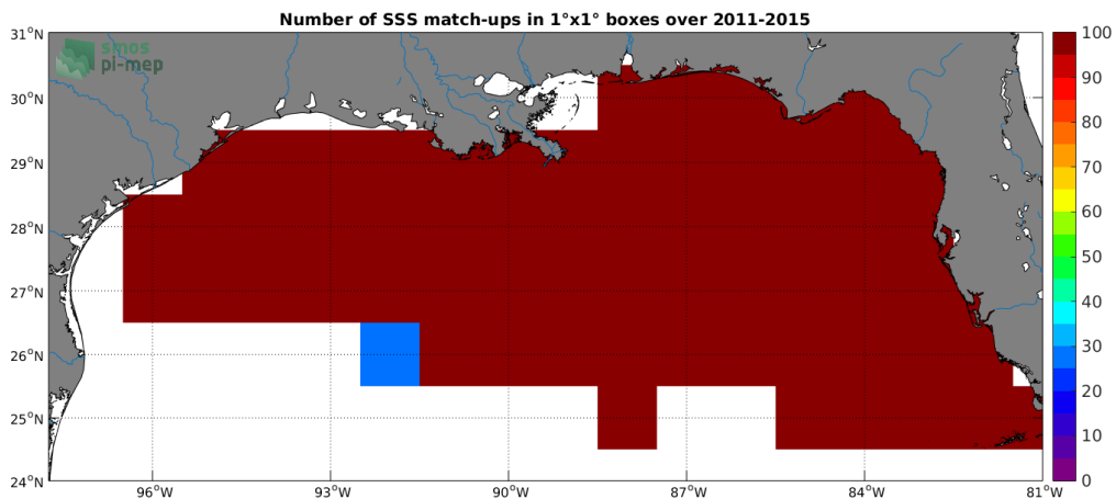
Figure 4: Number of SSS match-ups between TSG-SAMOS SSS and the Aquarius-L4-IPRC-V5-MONTHLY SSS product for the Mississippi river plume Pi-MEP region over 1^\circ \times 1^\circ boxes and for the full satellite product period.
