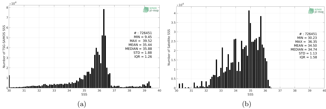
Figure 2: Histograms of SSS from TSG-SAMOS (a) and Aquarius-L4-IPRC-V5-MONTHLY (b) considering all match-up pairs per bins of 0.1 over the Mississippi river plume Pi-MEP region and for the full satellite product period.
