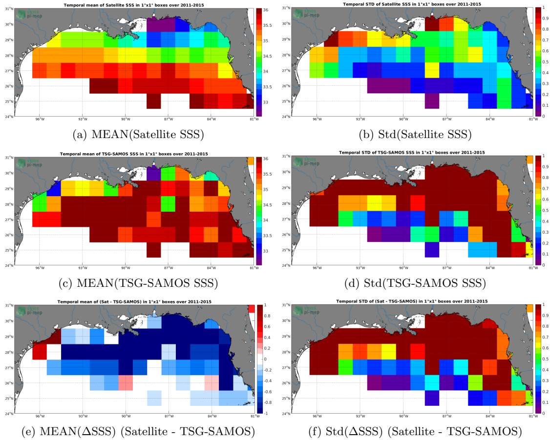
Figure 6: Temporal mean (left) and Std (right) of SSS from Aquarius-L4-IPRC-V5-MONTHLY (top), TSG-SAMOS (middle), and of \Delta SSS (Satellite - TSG-SAMOS). Only match-up pairs are used to generate these maps.
