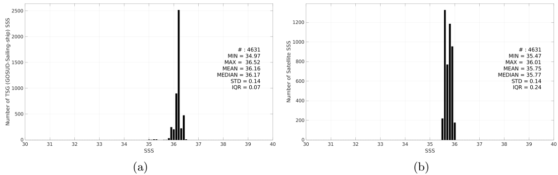
Figure 3: Histograms of SSS from TSG (GOSUD-Sailing-ship) (a) and Aquarius SSS L4 OI v5 - Monthly (IPRC) (b) considering all match-up pairs per bins of 0.1 over the Mississippi river plume Pi-MEP region and for the full satellite product period.
