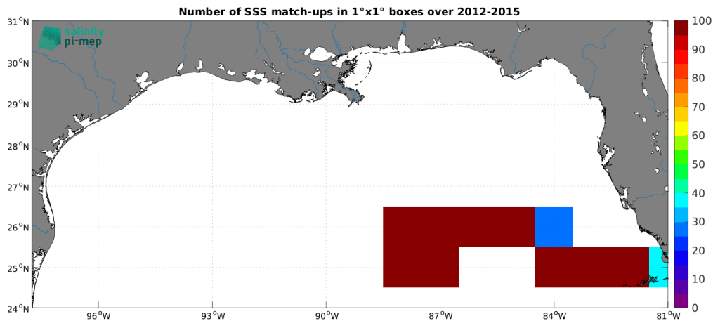
Figure 5: Number of SSS match-ups between TSG (GOSUD-Sailing-ship) SSS and the Aquarius SSS L4 OI v5 - Monthly (IPRC) SSS product for the Mississippi river plume Pi-MEP region over 1^\circ \times 1^\circ boxes and for the full satellite product period.
