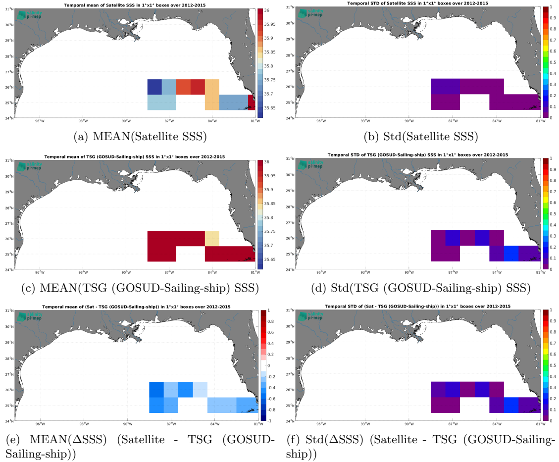
Figure 7: Temporal mean (left) and Std (right) of SSS from Aquarius SSS L4 OI v5 - Monthly (IPRC) (top), TSG (GOSUD-Sailing-ship) (middle), and of \Delta\text{SSS} (Satellite - TSG (GOSUD-Sailing-ship)). Only match-up pairs are used to generate these maps.
