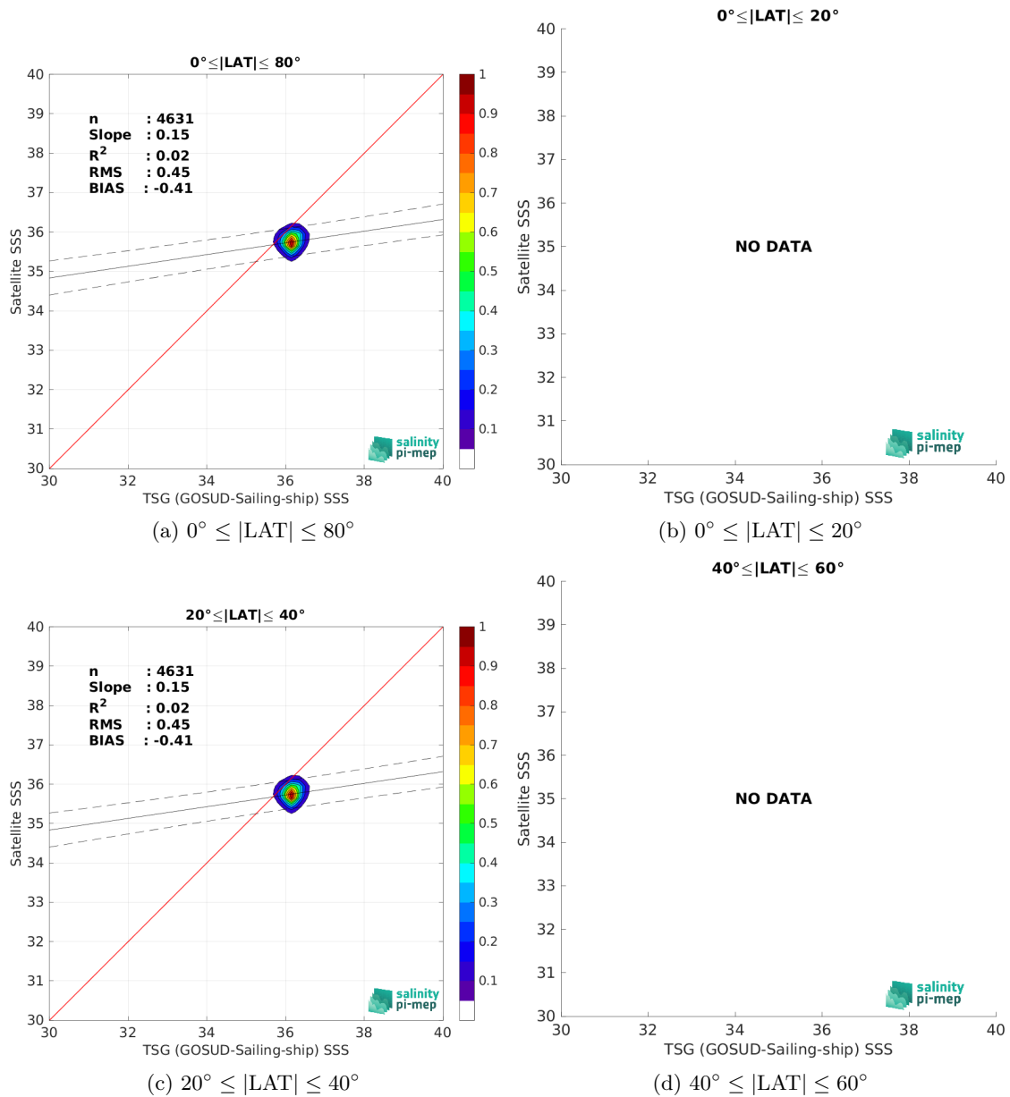
Figure 10: Contour maps of the concentration of Aquarius SSS L4 OI v5 - Monthly (IPRC) SSS (y-axis) versus TSG (GOSUD-Sailing-ship) SSS (x-axis) at match-up pairs for different latitude bands. For each plot, the red line shows x=y . The black thin and dashed lines indicate a linear fit through the data cloud and the \pm 95\% confidence levels, respectively. The number match-up pairs n , the slope and R^2 coefficient of the linear fit, the root mean square (RMS) and the mean bias between satellite and in situ data are indicated for each latitude band in each plots.
