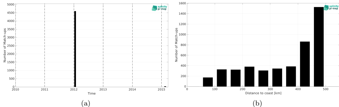
Figure 2: Number of match-ups between TSG (GOSUD-Sailing-ship) and Aquarius SSS L4 OI v5 - Monthly (IPRC) SSS as a function of time (a) and as function of the distance to coast (b) over the Mississippi river plume Pi-MEP region and for the full satellite product period.
