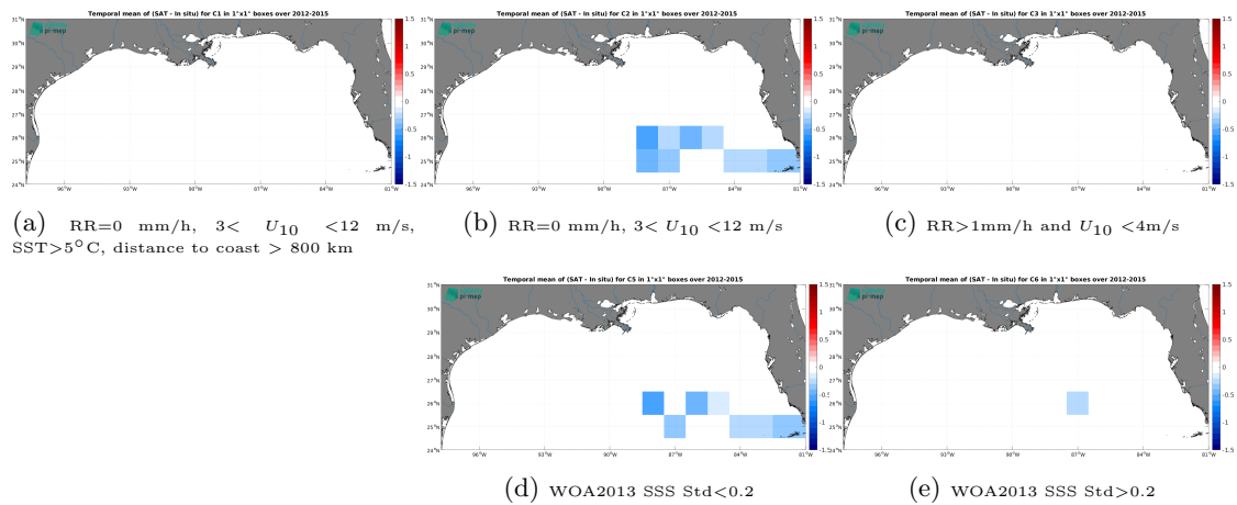
Figure 14: Temporal mean gridded over spatial boxes of size 1^\circ \times 1^\circ of \Delta SSS (Aquarius SSS L4 OI v5 - Monthly (IPRC) - TSG (GOSUD-Sailing-ship)) for 5 different subdatasets corresponding to: RR=0 mm/h, 3 < U_{10} < 12 m/s, SST > 5^\circ\text{C} , distance to coast > 800 km (a), RR=0 mm/h, 3 < U_{10} < 12 m/s (b), RR > 1 mm/h and U_{10} < 4 m/s (c), WOA2013 SSS Std < 0.2 (d), WOA2013 SSS Std > 0.2 (e).
