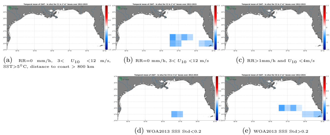
Figure 12: Temporal mean gridded over spatial boxes of size 1^\circ \times 1^\circ of \Delta SSS (Aquarius-L4-IPRC-V5-MONTHLY - TSG-GOSUD-Sailing-ship) for 5 different subdatasets corresponding to:RR=0 mm/h, 3 < U_{10} < 12 m/s, SST >5^\circ\text{C} , distance to coast > 800 km (a), RR=0 mm/h, 3 < U_{10} < 12 m/s (b), RR >1 mm/h and U_{10} < 4 m/s (c), WOA2013 SSS Std <0.2 (d), WOA2013 SSS Std >0.2 (e).
