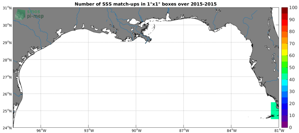
Figure 4: Number of SSS match-ups between TSG-GOSUD-Sailing-ship SSS and the Aquarius-L4-IPRC-V5-MONTHLY SSS product for the Mississippi river plume Pi-MEP region over 1^{\circ} \times 1^{\circ} boxes and for the full satellite product period.
