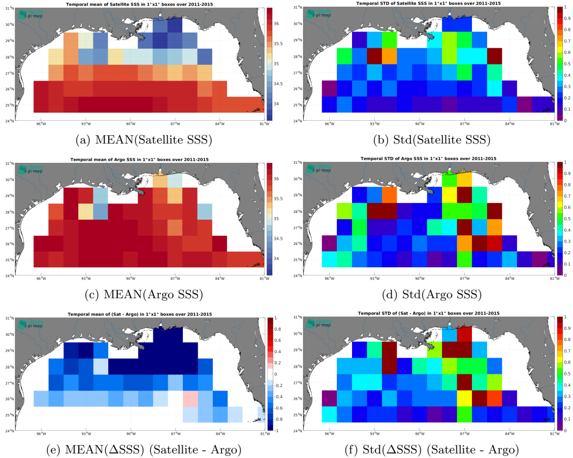
Figure 6: Temporal mean (left) and Std (right) of SSS from Aquarius SSS L4 OI v5 - Monthly (IPRC) (top), Argo (middle), and of \Delta\text{SSS} (Satellite - Argo). Only match-up pairs are used to generate these maps.
