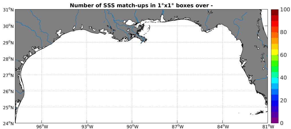
Figure 4: Number of SSS match-ups between TSG-SAMOS SSS and the Aquarius-L4-IPRC-V4-WEEKLY SSS product for the Mississippi river plume Pi-MEP region over 1^\circ \times 1^\circ boxes and for the full satellite product period.
