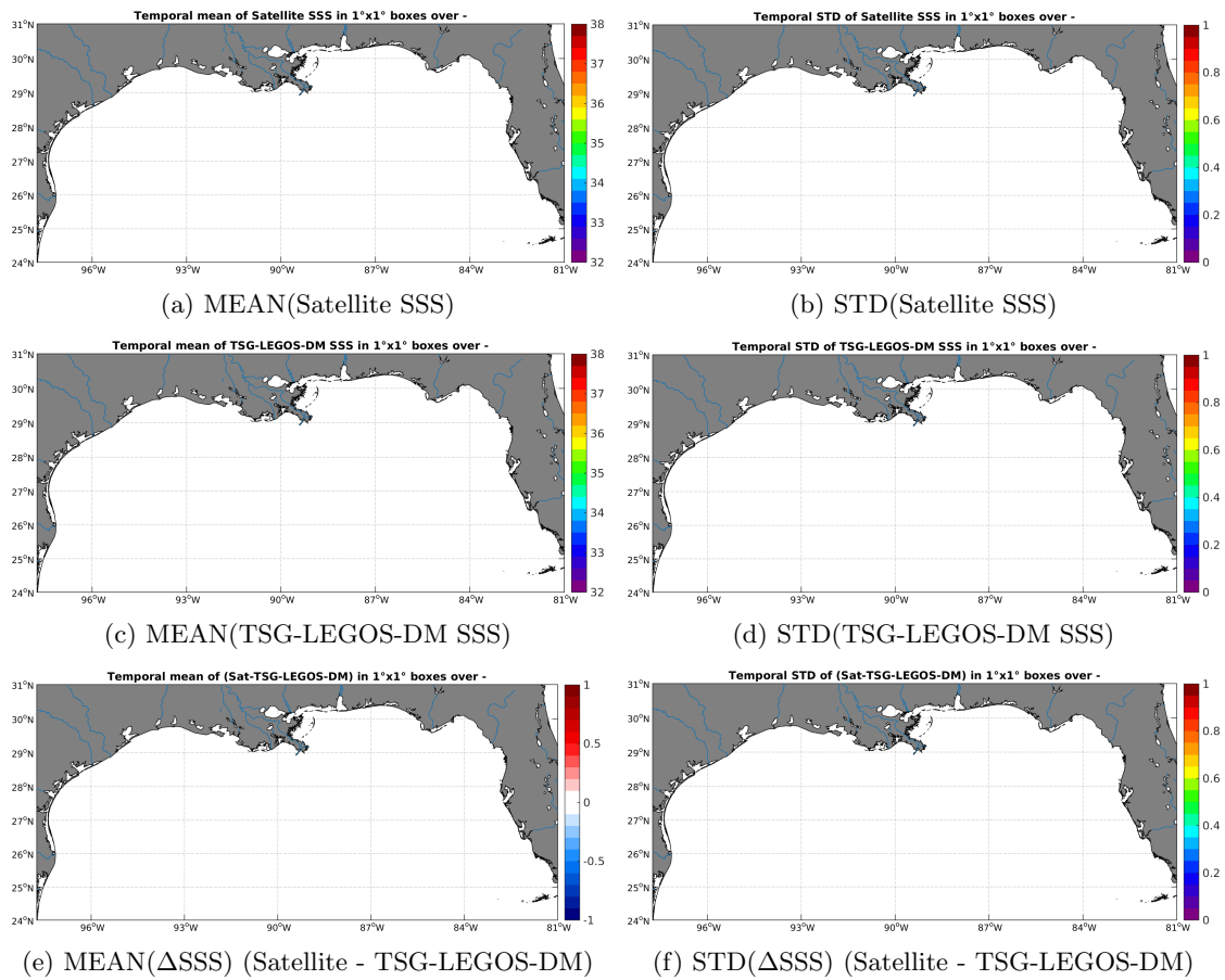
Figure 6: Temporal mean (left) and STD (right) of SSS from Aquarius-L4-IPRC-V4-WEEKLY (top), TSG-LEGOS-DM (middle), and of \Delta SSS (Satellite - TSG-LEGOS-DM). Only match-up pairs are used to generate these maps.
