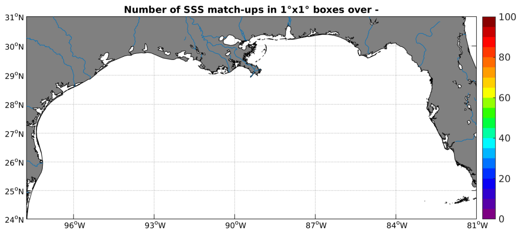
Figure 4: Number of SSS match-ups between TSG-LEGOS-DM SSS and the Aquarius-L4-IPRC-V4-WEEKLY SSS product for the Mississippi river plume Pi-MEP region over 1^\circ \times 1^\circ boxes and for the full satellite product period.
