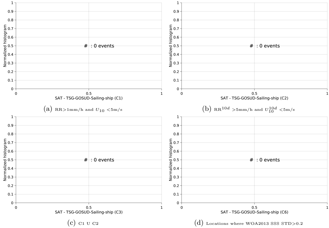
Figure 13: Normalized histogram of \Delta\text{SSS} (Aquarius-L4-IPRC-V4-WEEKLY - TSG-GOSUD-Sailing-ship) for 6 different subdatasets corresponding to: RR > 1\text{mm/h} and U_{10} < 5\text{m/s} (a), RR^{10d} > 5\text{mm/h} and U_{10}^{10d} < 5\text{m/s} (b), C1 U C2 (c), Locations where WOA2013 SSS STD > 0.2 (d).
