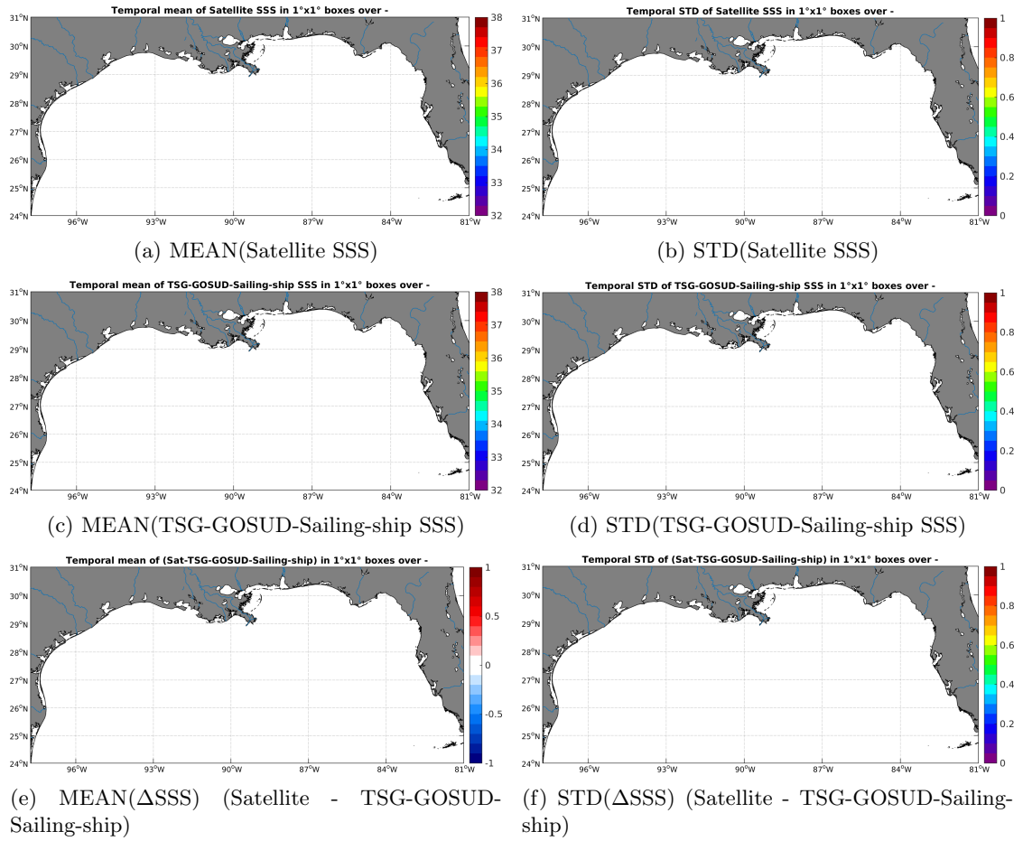
Figure 6: Temporal mean (left) and STD (right) of SSS from Aquarius-L4-IPRC-V4-WEEKLY (top), TSG-GOSUD-Sailing-ship (middle), and of \Delta SSS (Satellite - TSG-GOSUD-Sailing-ship). Only match-up pairs are used to generate these maps.
