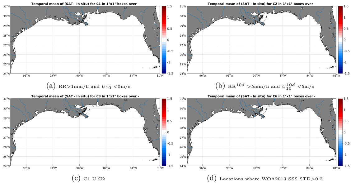
Figure 12: Temporal mean gridded over spatial boxes of size 1^\circ \times 1^\circ of \Delta SSS (Aquarius-L4-IPRC-V4-WEEKLY - TSG-GOSUD-Research-vessel) for 4 different subdatasets corresponding to:RR > 1 mm/h and U_{10} < 5 m/s (a), RR^{10d} > 5 mm/h and U_{10}^{10d} < 5 m/s (b), C1 U C2 (c),Locations where WOA2013 SSS STD > 0.2 (d).
