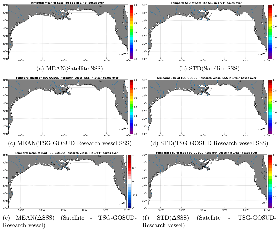
Figure 6: Temporal mean (left) and STD (right) of SSS from Aquarius-L4-IPRC-V4-WEEKLY (top), TSG-GOSUD-Research-vessel (middle), and of \Delta SSS (Satellite - TSG-GOSUD-Research-vessel). Only match-up pairs are used to generate these maps.
