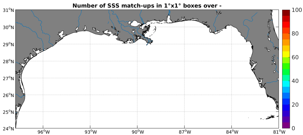
Figure 4: Number of SSS match-ups between TSG-GOSUD-Research-vessel SSS and the Aquarius-L4-IPRC-V4-WEEKLY SSS product for the Mississippi river plume Pi-MEP region over 1^\circ \times 1^\circ boxes and for the full satellite product period.
