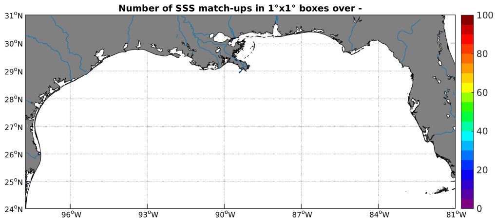
Figure 4: Number of SSS match-ups between Argo SSS and the Aquarius-L4-IPRC-V4-WEEKLY SSS product for the Mississippi river plume Pi-MEP region over 1^\circ \times 1^\circ boxes and for the full satellite product period.
