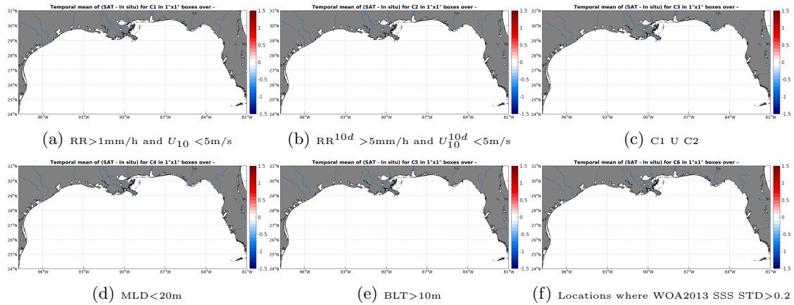
Figure 12: Temporal mean gridded over spatial boxes of size 1^\circ \times 1^\circ of \Delta SSS (Aquarius-L4-IPRC-V4-WEEKLY - Argo) for 6 different subdatasets corresponding to:RR>1mm/h and U_{10} < 5\text{m/s} (a), RR^{10d} > 5\text{mm/h} and U_{10}^{10d} < 5\text{m/s} (b), C1 U C2 (c),MLD<20m (d),BLT>10m (e),Locations where WOA2013 SSS STD>0.2 (f).
