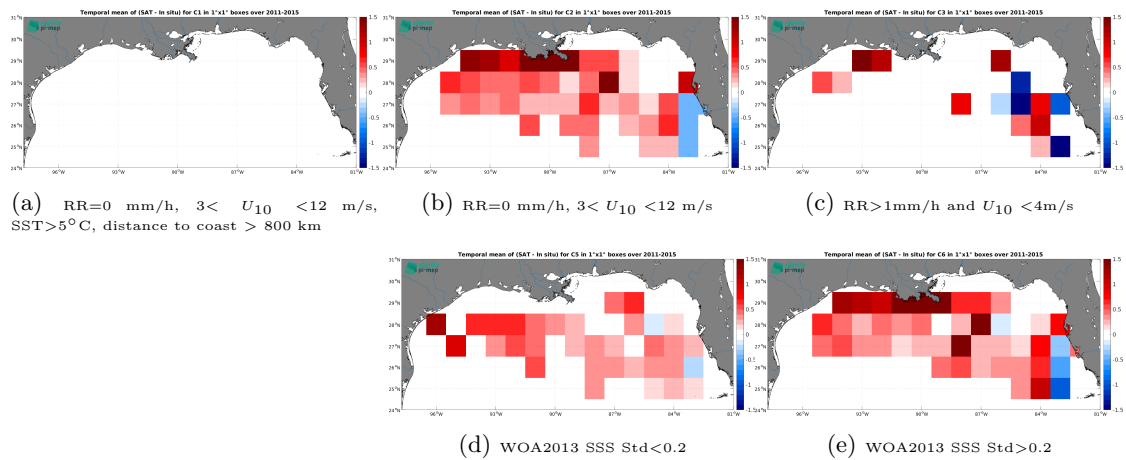
Figure 14: Temporal mean gridded over spatial boxes of size 1^\circ \times 1^\circ of \Delta\text{SSS} (Aquarius SSS L3 CAP v5 - 7-Day running (JPL) - TSG (SAMOS)) for 5 different subdatasets corresponding to:RR=0 mm/h, 3 < U_{10} < 12 m/s, SST >5^\circ\text{C} , distance to coast > 800 km (a), RR=0 mm/h, 3 < U_{10} < 12 m/s (b), RR >1 mm/h and U_{10} < 4 m/s (c), WOA2013 SSS Std <0.2 (d), WOA2013 SSS Std >0.2 (e).
