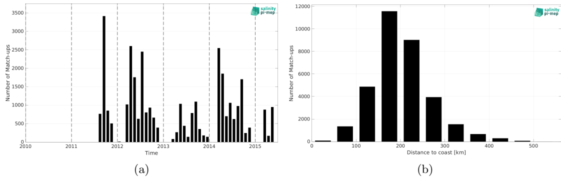
Figure 2: Number of match-ups between TSG (SAMOS) and Aquarius SSS L3 CAP v5 - 7-Day running (JPL) SSS as a function of time (a) and as function of the distance to coast (b) over the Mississippi river plume Pi-MEP region and for the full satellite product period.
