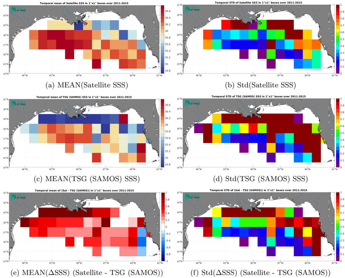
Figure 7: Temporal mean (left) and Std (right) of SSS from Aquarius SSS L3 CAP v5 - 7-Day running (JPL) (top), TSG (SAMOS) (middle), and of \Delta SSS (Satellite - TSG (SAMOS)). Only match-up pairs are used to generate these maps.
