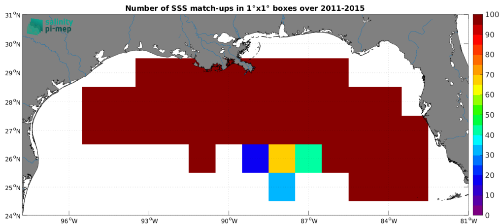
Figure 5: Number of SSS match-ups between TSG (SAMOS) SSS and the Aquarius SSS L3 CAP v5 - 7-Day running (JPL) SSS product for the Mississippi river plume Pi-MEP region over 1^\circ \times 1^\circ boxes and for the full satellite product period.
