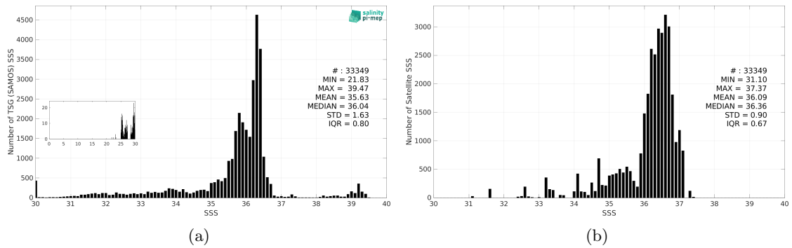
Figure 3: Histograms of SSS from TSG (SAMOS) (a) and Aquarius SSS L3 CAP v5 - 7-Day running (JPL) (b) considering all match-up pairs per bins of 0.1 over the Mississippi river plume Pi-MEP region and for the full satellite product period.
