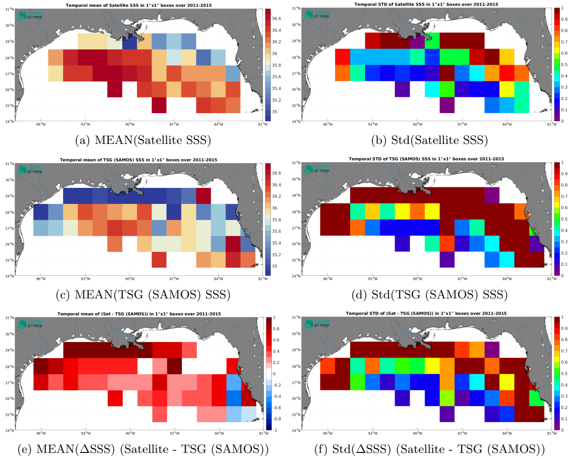
Figure 6: Temporal mean (left) and Std (right) of SSS from Aquarius SSS L3 CAP v5 - 7-Day running (JPL) (top), TSG (SAMOS) (middle), and of \Delta SSS (Satellite - TSG (SAMOS)). Only match-up pairs are used to generate these maps.
