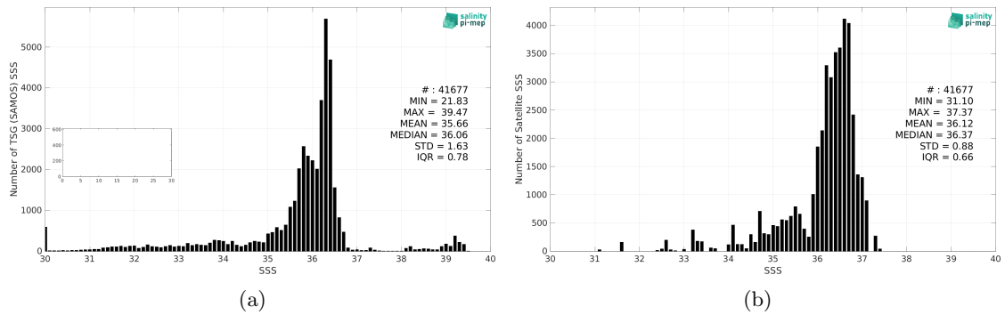
Figure 2: Histograms of SSS from TSG (SAMOS) (a) and Aquarius SSS L3 CAP v5 - 7-Day running (JPL) (b) considering all match-up pairs per bins of 0.1 over the Mississippi river plume Pi-MEP region and for the full satellite product period.
