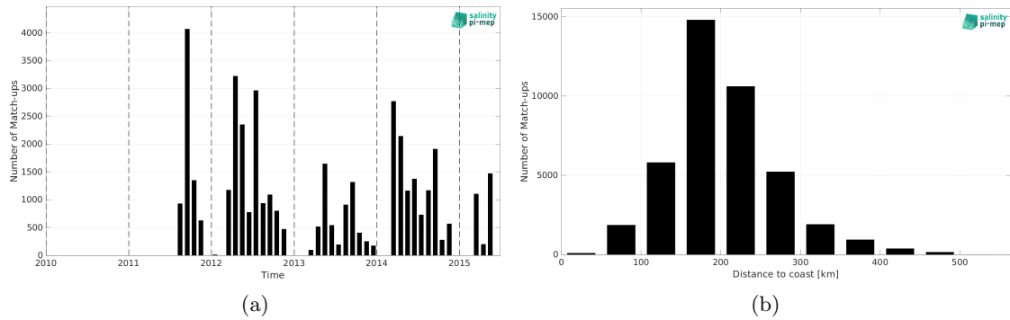
Figure 1: Number of match-ups between TSG (SAMOS) and Aquarius SSS L3 CAP v5 - 7-Day running (JPL) SSS as a function of time (a) and as function of the distance to coast (b) over the Mississippi river plume Pi-MEP region and for the full satellite product period.
