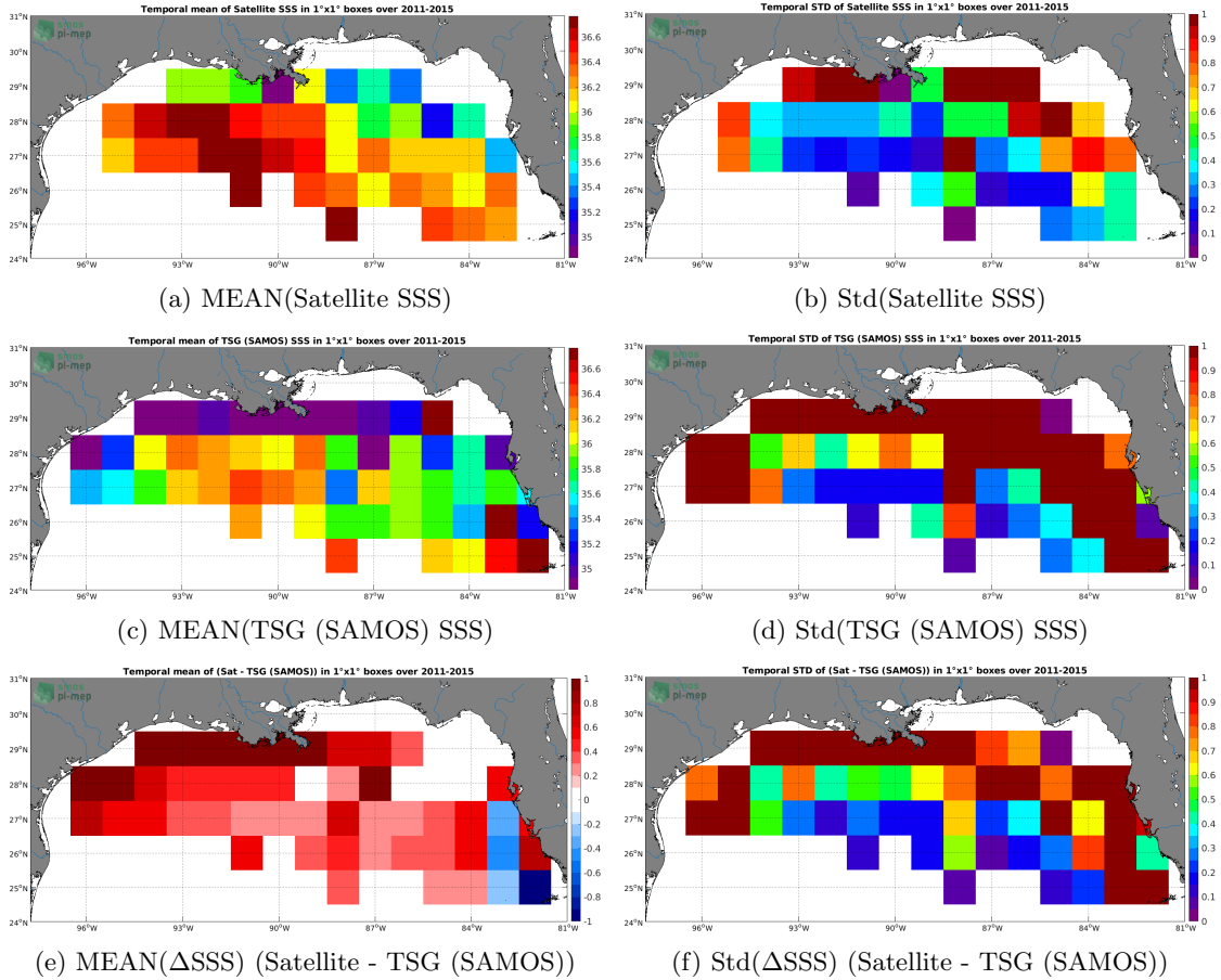
Figure 6: Temporal mean (left) and Std (right) of SSS from Aquarius SSS L3 CAP v5 - 7-Day running (JPL) (top), TSG (SAMOS) (middle), and of \Delta\text{SSS} (Satellite - TSG (SAMOS)). Only match-up pairs are used to generate these maps.
