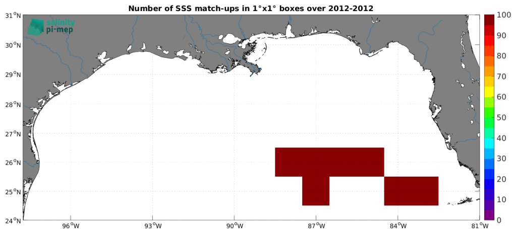
Figure 5: Number of SSS match-ups between TSG (GOSUD-Sailing-ship) SSS and the Aquarius SSS L3 CAP v5 - 7-Day running (JPL) SSS product for the Mississippi river plume Pi-MEP region over 1^\circ \times 1^\circ boxes and for the full satellite product period.
