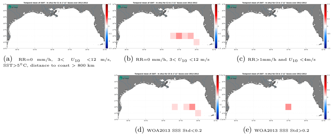
Figure 14: Temporal mean gridded over spatial boxes of size 1^\circ \times 1^\circ of \Delta SSS (Aquarius SSS L3 CAP v5 - 7-Day running (JPL) - TSG (GOSUD-Sailing-ship)) for 5 different subdatasets corresponding to:RR=0 mm/h, 3 < U_{10} < 12 m/s, SST >5^\circ\text{C} , distance to coast > 800 km (a), RR=0 mm/h, 3 < U_{10} < 12 m/s (b), RR >1 mm/h and U_{10} < 4 m/s (c), WOA2013 SSS Std <0.2 (d), WOA2013 SSS Std >0.2 (e).
