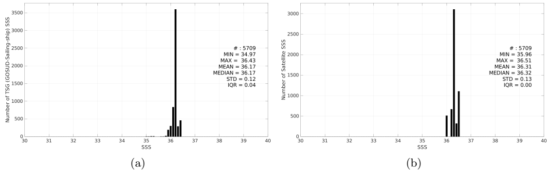
Figure 3: Histograms of SSS from TSG (GOSUD-Sailing-ship) (a) and Aquarius SSS L3 CAP v5 - 7-Day running (JPL) (b) considering all match-up pairs per bins of 0.1 over the Mississippi river plume Pi-MEP region and for the full satellite product period.
