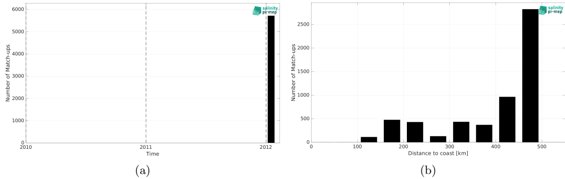
Figure 2: Number of match-ups between TSG (GOSUD-Sailing-ship) and Aquarius SSS L3 CAP v5 - 7-Day running (JPL) SSS as a function of time (a) and as function of the distance to coast (b) over the Mississippi river plume Pi-MEP region and for the full satellite product period.
