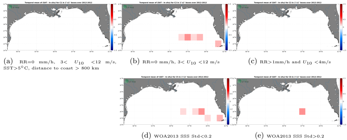
Figure 12: Temporal mean gridded over spatial boxes of size 1^{\circ}\times 1^{\circ} of \Delta SSS (Aquarius SSS L3 CAP v5 - 7-Day running (JPL) - TSG (GOSUD-Sailing-ship)) for 5 different subdatasets corresponding to:RR=0 mm/h, 3 < U_{10} < 12 m/s, SST >5^{\circ}\text{C} , distance to coast > 800 km (a), RR=0 mm/h, 3 < U_{10} < 12 m/s (b), RR >1 mm/h and U_{10} < 4 m/s (c), WOA2013 SSS Std <0.2 (d), WOA2013 SSS Std >0.2 (e).
