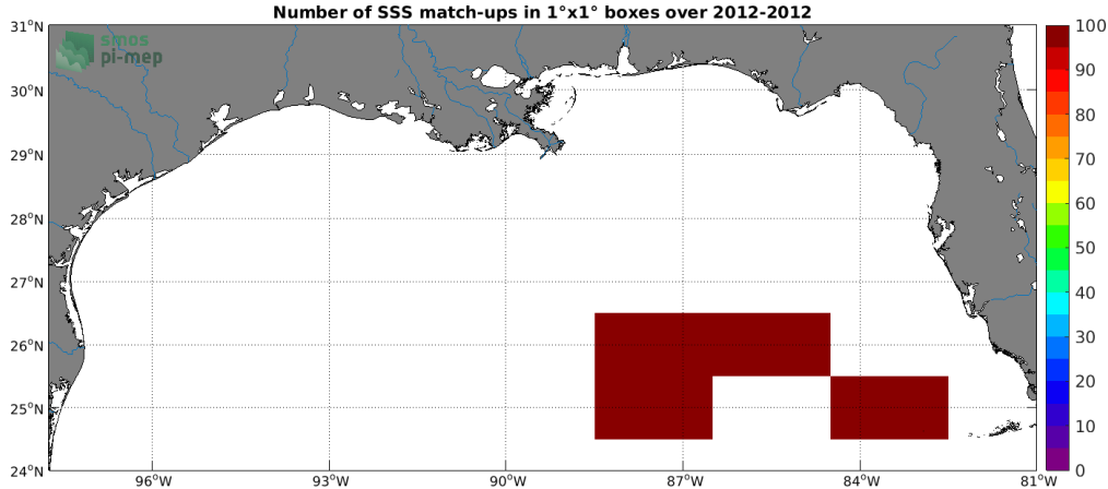
Figure 4: Number of SSS match-ups between TSG (GOSUD-Sailing-ship) SSS and the Aquarius SSS L3 CAP v5 - 7-Day running (JPL) SSS product for the Mississippi river plume Pi-MEP region over 1°x1° boxes and for the full satellite product period.
