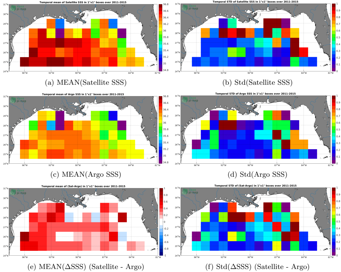
Figure 6: Temporal mean (left) and Std (right) of SSS from Aquarius-L3-JPL-V5-7DAY-RUNNING (top), Argo (middle), and of \Delta\text{SSS} (Satellite - Argo). Only match-up pairs are used to generate these maps.
