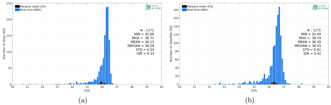
Figure 2: Histograms of SSS from Argos (a) and Aquarius-L3-JPL-V5-7DAY-RUNNING (b) considering all match-up pairs per bins of 0.1 over the Mississippi river plume Pi-MEP region and for the full satellite product period.
