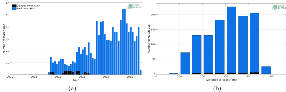
Figure 1: Number of match-ups between Argo and Aquarius-L3-JPL-V5-7DAY-RUNNING SSS as a function of time (a) and as function of the distance to coast (b) over the Mississippi river plume Pi-MEP region and for the full satellite product period.
