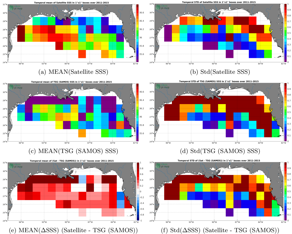
Figure 6: Temporal mean (left) and Std (right) of SSS from Aquarius SSS L3 CAP v5 - Monthly (JPL) (top), TSG (SAMOS) (middle), and of \Delta\text{SSS} (Satellite - TSG (SAMOS)). Only match-up pairs are used to generate these maps.
