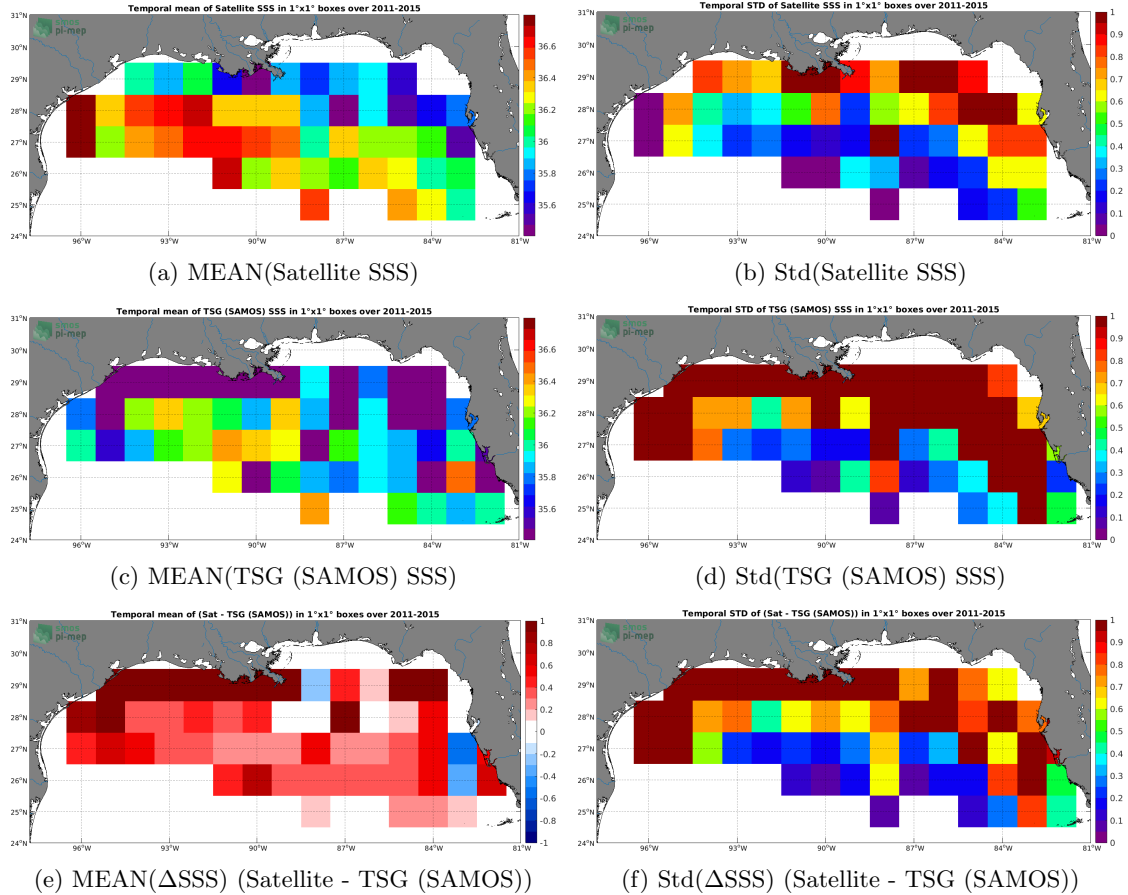
Figure 6: Temporal mean (left) and Std (right) of SSS from Aquarius SSS L3 CAP v5 - Monthly (JPL) (top), TSG (SAMOS) (middle), and of \Delta\text{SSS} (Satellite - TSG (SAMOS)). Only match-up pairs are used to generate these maps.
