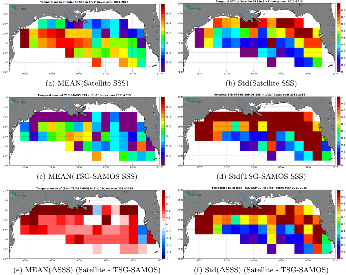
Figure 6: Temporal mean (left) and Std (right) of SSS from Aquarius-L3-JPL-V5-MONTHLY (top), TSG-SAMOS (middle), and of \Delta\text{SSS}(\text{Satellite} - \text{TSG-SAMOS}) . Only match-up pairs are used to generate these maps.
