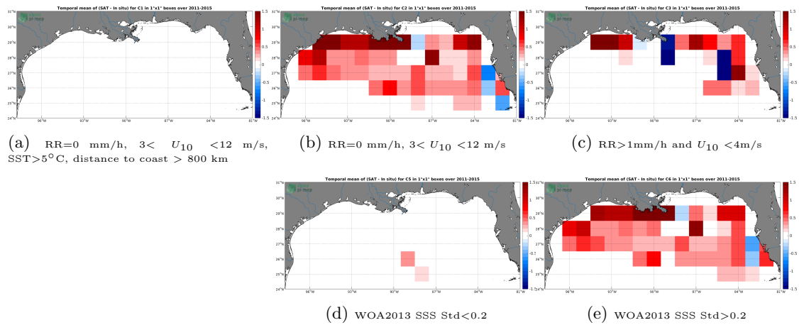
Figure 12: Temporal mean gridded over spatial boxes of size 1^\circ \times 1^\circ of \Delta SSS (Aquarius-L3-JPL-V5-MONTHLY - TSG-SAMOS) for 5 different subdatasets corresponding to:RR=0 mm/h, 3 < U_{10} < 12 m/s, SST >5^\circ\text{C} , distance to coast > 800 km (a), RR=0 mm/h, 3 < U_{10} < 12 m/s (b), RR >1 mm/h and U_{10} < 4 m/s (c), WOA2013 SSS Std <0.2 (d), WOA2013 SSS Std >0.2 (e).
