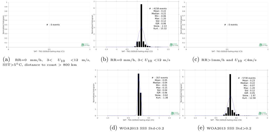
Figure 13: Normalized histogram of \Delta SSS (Aquarius SSS L3 CAP v5 - Monthly (JPL) - TSG (GOSUD-Sailing-ship)) for 5 different subdatasets corresponding to: RR=0 mm/h, 3 < U_{10} < 12 m/s, SST > 5°C, distance to coast > 800 km (a), RR=0 mm/h, 3 < U_{10} < 12 m/s (b), RR > 1mm/h and U_{10} < 4 m/s (c), WOA2013 SSS Std < 0.2 (d), WOA2013 SSS Std > 0.2 (e).
