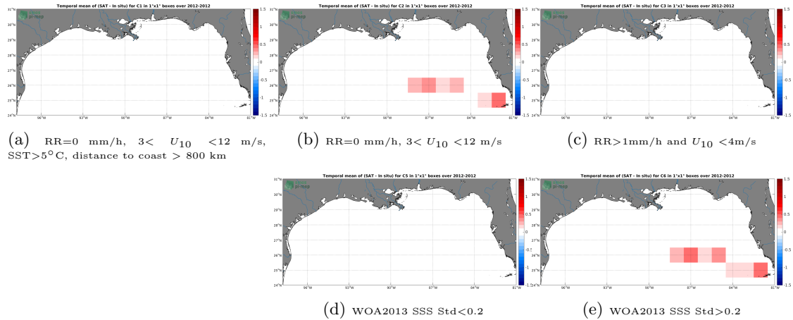
Figure 12: Temporal mean gridded over spatial boxes of size 1^\circ \times 1^\circ of \Delta SSS (Aquarius SSS L3 CAP v5 - Monthly (JPL) - TSG (GOSUD-Sailing-ship)) for 5 different subdatasets corresponding to: RR=0 mm/h, 3 < U_{10} < 12 m/s, SST > 5^\circ\text{C} , distance to coast > 800 km (a), RR=0 mm/h, 3 < U_{10} < 12 m/s (b), RR > 1 mm/h and U_{10} < 4 m/s (c), WOA2013 SSS Std < 0.2 (d), WOA2013 SSS Std > 0.2 (e).
