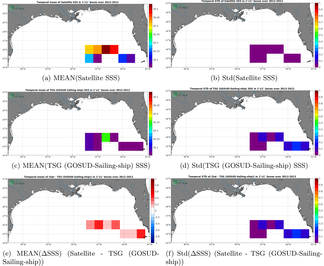
Figure 6: Temporal mean (left) and Std (right) of SSS from Aquarius SSS L3 CAP v5 - Monthly (JPL) (top), TSG (GOSUD-Sailing-ship) (middle), and of \Delta\text{SSS} (Satellite - TSG (GOSUD-Sailing-ship)). Only match-up pairs are used to generate these maps.
