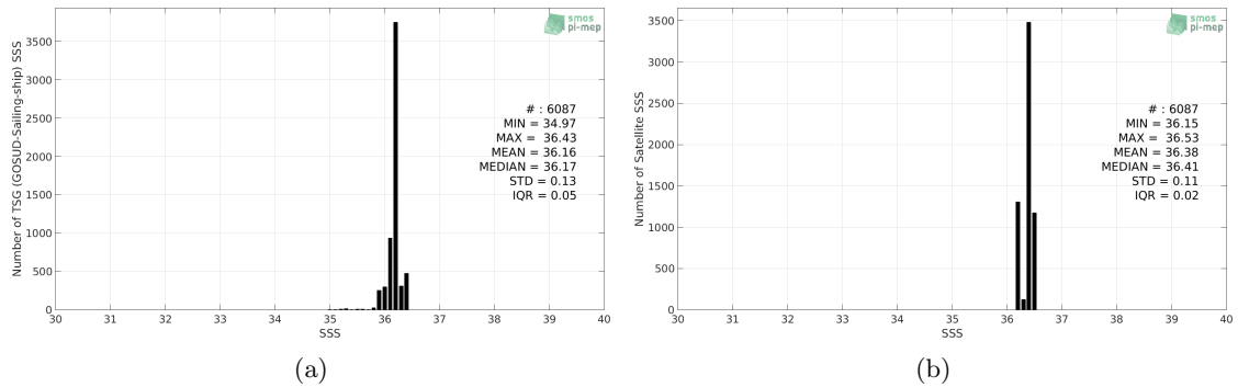
Figure 2: Histograms of SSS from TSG (GOSUD-Sailing-ship) (a) and Aquarius SSS L3 CAP v5 - Monthly (JPL) (b) considering all match-up pairs per bins of 0.1 over the Mississippi river plume Pi-MEP region and for the full satellite product period.
