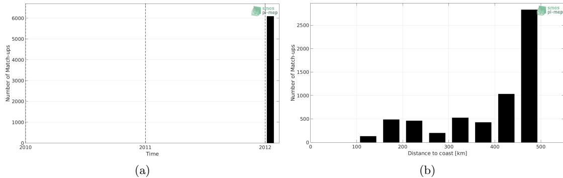
Figure 1: Number of match-ups between TSG (GOSUD-Sailing-ship) and Aquarius SSS L3 CAP v5 - Monthly (JPL) SSS as a function of time (a) and as function of the distance to coast (b) over the Mississippi river plume Pi-MEP region and for the full satellite product period.
