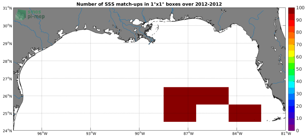
Figure 4: Number of SSS match-ups between TSG (GOSUD-Sailing-ship) SSS and the Aquarius SSS L3 CAP v5 - Monthly (JPL) SSS product for the Mississippi river plume Pi-MEP region over 1^\circ \times 1^\circ boxes and for the full satellite product period.
