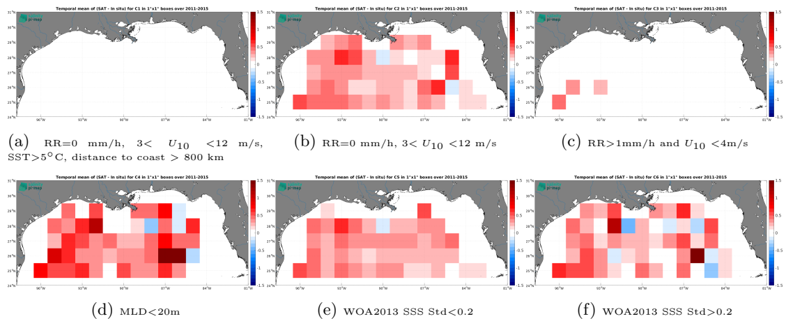
Figure 14: Temporal mean gridded over spatial boxes of size 1^\circ \times 1^\circ of \Delta SSS (Aquarius SSS L3 CAP v5 - Monthly (JPL) - Argo) for 6 different subdatasets corresponding to:RR=0 mm/h, 3 < U_{10} < 12 m/s, SST >5^\circ C, distance to coast > 800 km (a), RR=0 mm/h, 3 < U_{10} < 12 m/s (b), RR >1 mm/h and U_{10} < 4 m/s (c),MLD <20 m (d),WOA2013 SSS Std <0.2 (e),WOA2013 SSS Std >0.2 (f).
