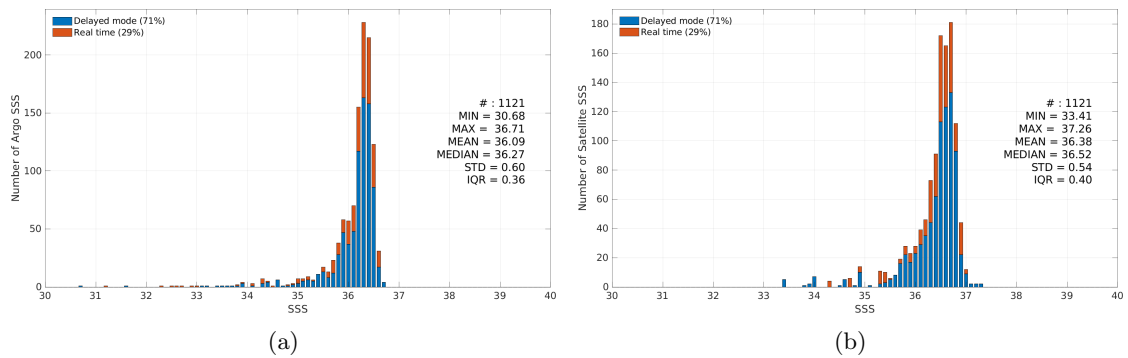
Figure 3: Histograms of SSS from Argo (a) and Aquarius SSS L3 CAP v5 - Monthly (JPL) (b) considering all match-up pairs per bins of 0.1 over the Mississippi river plume Pi-MEP region and for the full satellite product period.
