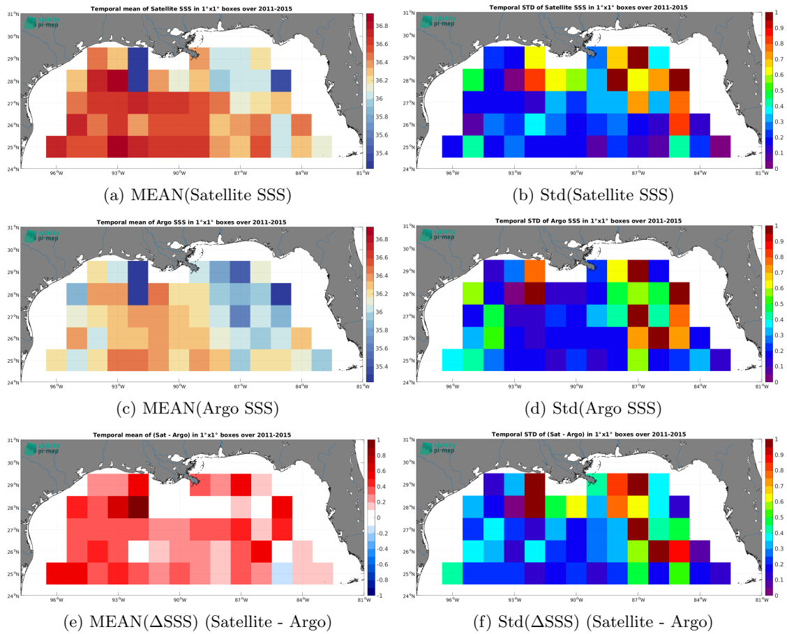
Figure 7: Temporal mean (left) and Std (right) of SSS from Aquarius SSS L3 CAP v5 - Monthly (JPL) (top), Argo (middle), and of \Delta SSS (Satellite - Argo). Only match-up pairs are used to generate these maps.
