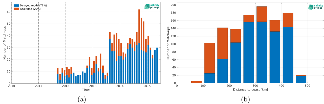
Figure 2: Number of match-ups between Argo and Aquarius SSS L3 CAP v5 - Monthly (JPL) SSS as a function of time (a) and as function of the distance to coast (b) over the Mississippi river plume Pi-MEP region and for the full satellite product period.
