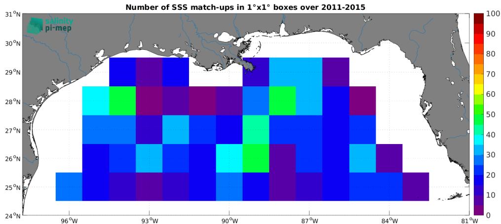
Figure 5: Number of SSS match-ups between Argo SSS and the Aquarius SSS L3 CAP v5 - Monthly (JPL) SSS product for the Mississippi river plume Pi-MEP region over 1^\circ \times 1^\circ boxes and for the full satellite product period.
