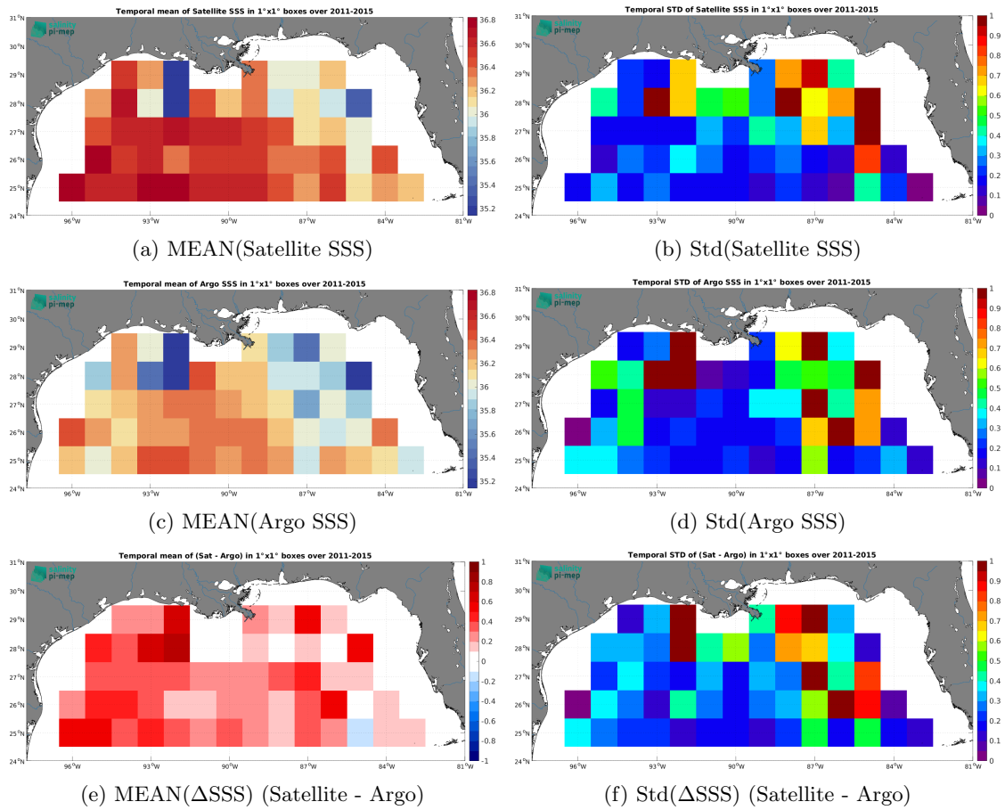
Figure 6: Temporal mean (left) and Std (right) of SSS from Aquarius SSS L3 CAP v5 - Monthly (JPL) (top), Argo (middle), and of \Delta SSS (Satellite - Argo). Only match-up pairs are used to generate these maps.
