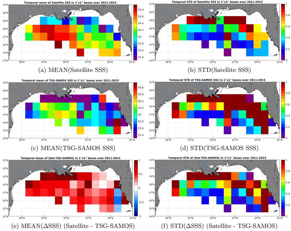
Figure 6: Temporal mean (left) and STD (right) of SSS from Aquarius-L3-JPL-V4-7DAY-RUNNING (top), TSG-SAMOS (middle), and of \Delta SSS (Satellite - TSG-SAMOS). Only match-up pairs are used to generate these maps.
