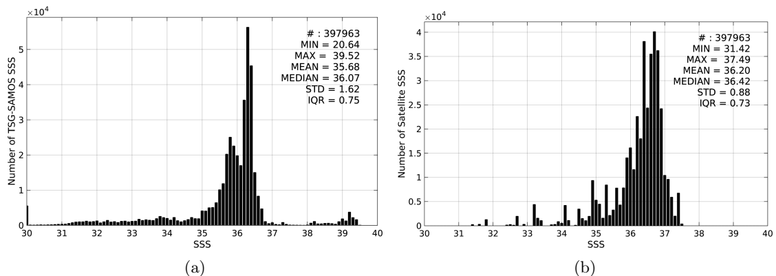
Figure 2: Histograms of SSS from TSG-SAMOS (a) and Aquarius-L3-JPL-V4-7DAY-RUNNING (b) considering all match-up pairs per bins of 0.1 over the Mississippi river plume Pi-MEP region and for the full satellite product period.
