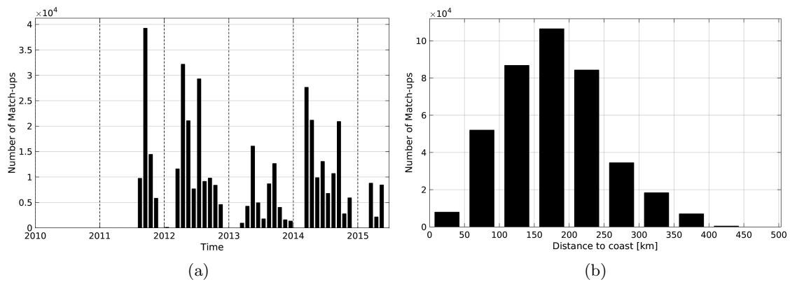
Figure 1: Number of match-ups between TSG-SAMOS and Aquarius-L3-JPL-V4-7DAY-RUNNING SSS as a function of time (a) and as function of the distance to coast (b) over the Mississippi river plume Pi-MEP region and for the full satellite product period.
