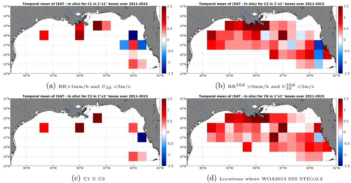
Figure 12: Temporal mean gridded over spatial boxes of size 1^\circ \times 1^\circ of \Delta SSS (Aquarius-L3-JPL-V4-7DAY-RUNNING - TSG-SAMOS) for 4 different subdatasets corresponding to: RR > 1\text{mm/h} and U_{10} < 5\text{m/s} (a), RR^{10d} > 5\text{mm/h} and U_{10}^{10d} < 5\text{m/s} (b), C1 U C2 (c), Locations where WOA2013 SSS STD > 0.2 (d).
