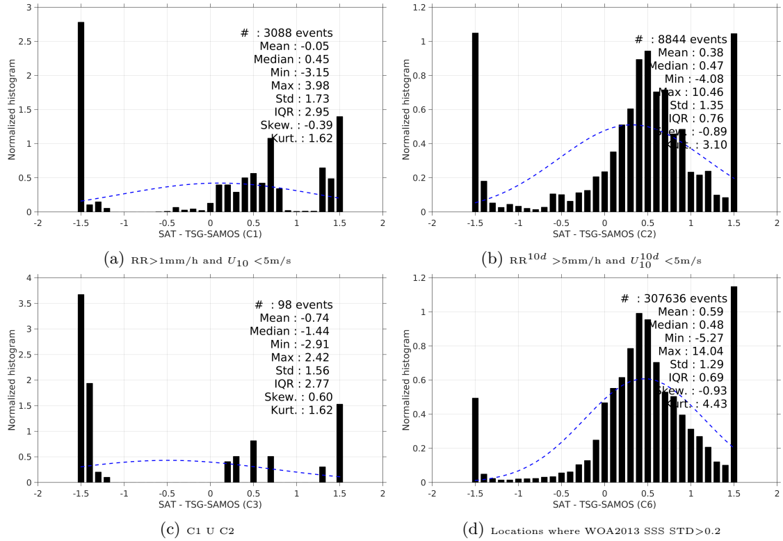
Figure 13: Normalized histogram of \Delta\text{SSS} (Aquarius-L3-JPL-V4-7DAY-RUNNING - TSG-SAMOS) for 6 different subdatasets corresponding to: RR>1mm/h and U_{10} < 5\text{m/s} (a), RR^{10d} > 5\text{mm/h} and U_{10}^{10d} < 5\text{m/s} (b), C1 U C2 (c), Locations where WOA2013 SSS STD>0.2 (d).
