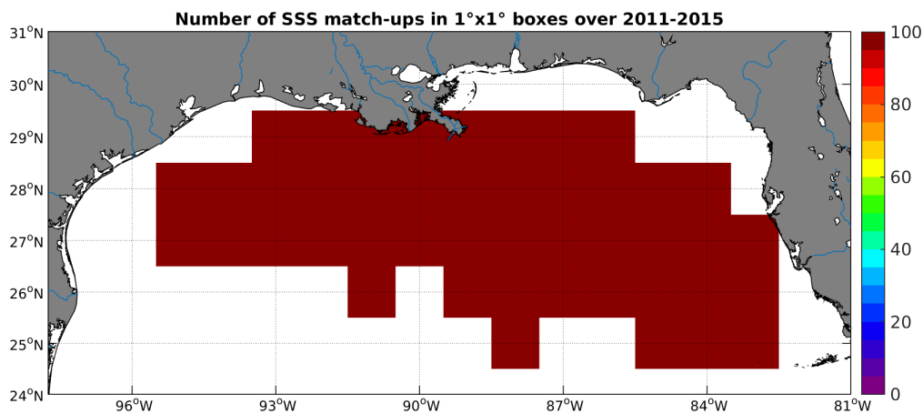
Figure 4: Number of SSS match-ups between TSG-SAMOS SSS and the Aquarius-L3-JPL-V4-7DAY-RUNNING SSS product for the Mississippi river plume Pi-MEP region over 1^\circ \times 1^\circ boxes and for the full satellite product period.
