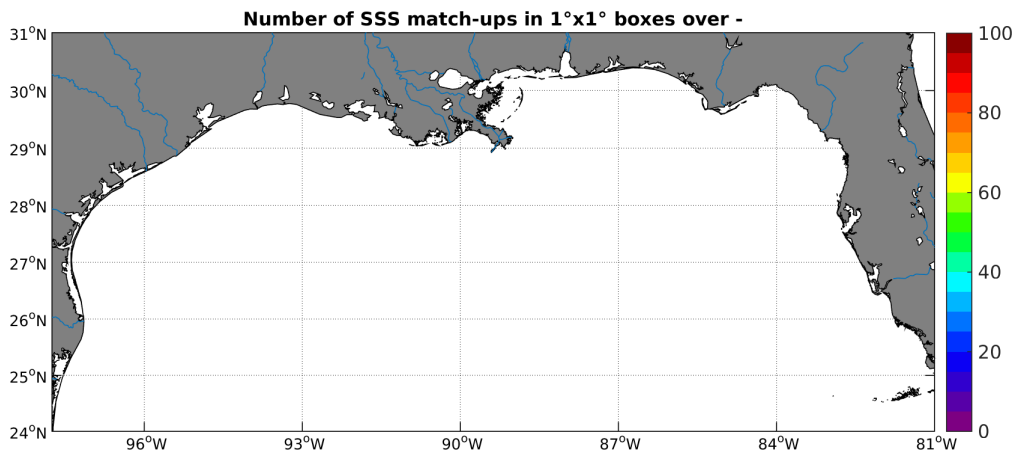
Figure 4: Number of SSS match-ups between TSG-LEGOS-DM SSS and the Aquarius-L3-JPL-V4-7DAY-RUNNING SSS product for the Mississippi river plume Pi-MEP region over 1^\circ \times 1^\circ boxes and for the full satellite product period.
