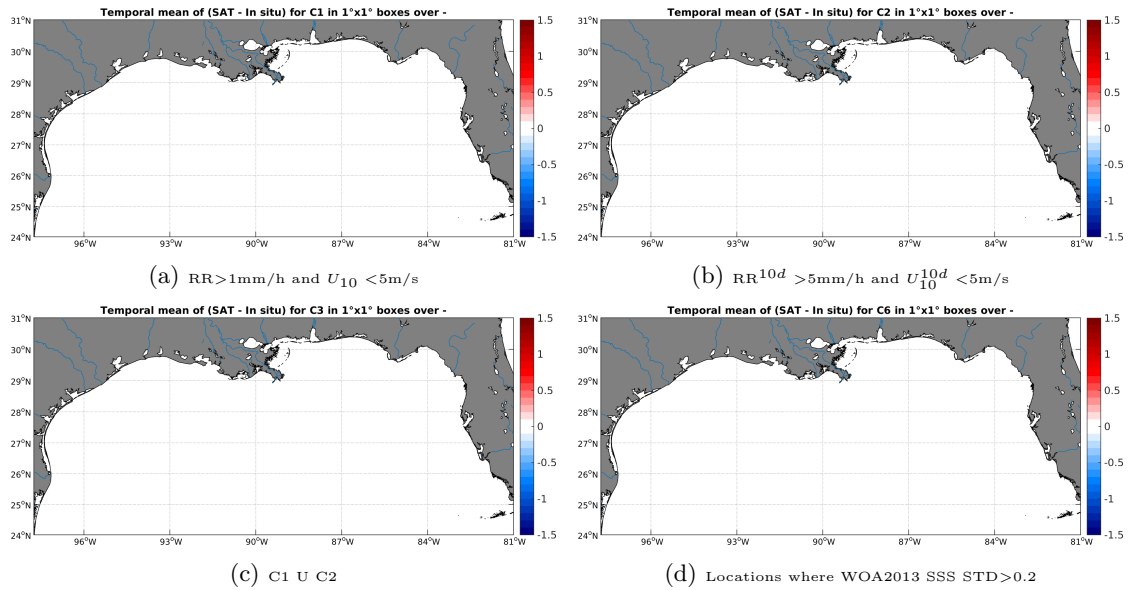
Figure 12: Temporal mean gridded over spatial boxes of size 1^\circ \times 1^\circ of \Delta SSS (Aquarius-L3-JPL-V4-7DAY-RUNNING - TSG-LEGOS-DM) for 4 different subdatasets corresponding to:RR > 1 mm/h and U_{10} < 5 m/s (a), RR^{10d} > 5 mm/h and U_{10}^{10d} < 5 m/s (b), C1 U C2 (c),Locations where WOA2013 SSS STD > 0.2 (d).
