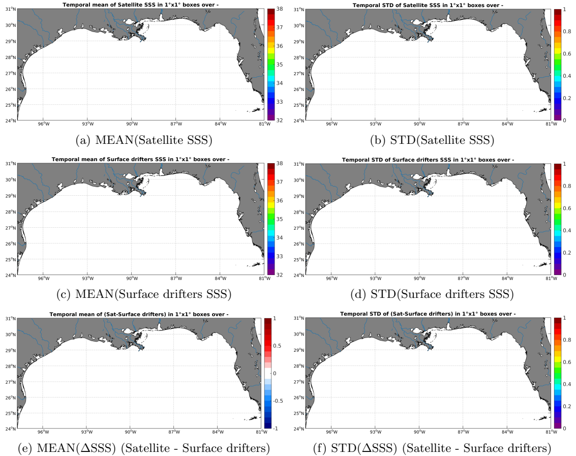
Figure 5: Temporal mean (left) and STD (right) of SSS from Aquarius-L3-JPL-V4-7DAY-RUNNING (top), Surface drifters (middle), and of \Delta SSS (Satellite - Surface drifters). Only match-up pairs are used to generate these maps.
