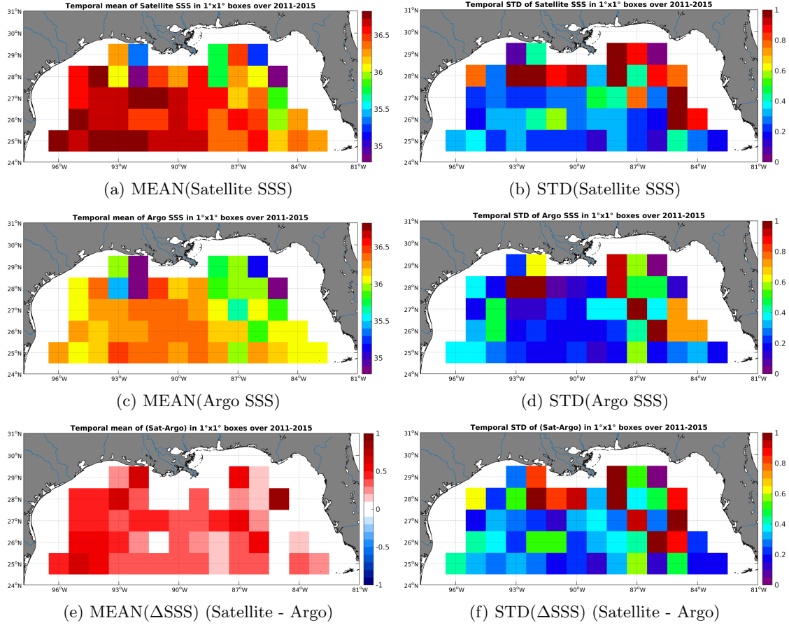
Figure 6: Temporal mean (left) and STD (right) of SSS from Aquarius-L3-JPL-V4-7DAY-RUNNING (top), Argo (middle), and of \Delta\text{SSS} (Satellite - Argo). Only match-up pairs are used to generate these maps.
