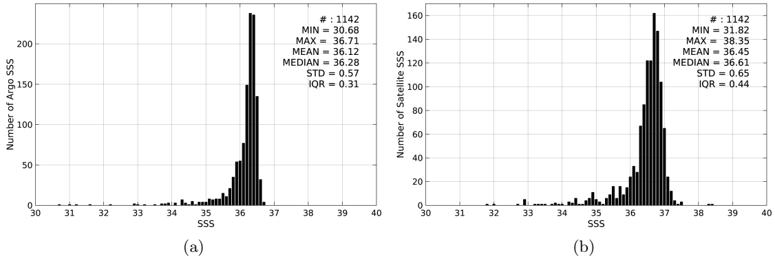
Figure 2: Histograms of SSS from Argo (a) and Aquarius-L3-JPL-V4-7DAY-RUNNING (b) considering all match-up pairs per bins of 0.1 over the Mississippi river plume Pi-MEP region and for the full satellite product period.
