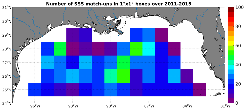
Figure 4: Number of SSS match-ups between Argo SSS and the Aquarius-L3-JPL-V4-7DAY-RUNNING SSS product for the Mississippi river plume Pi-MEP region over 1^\circ \times 1^\circ boxes and for the full satellite product period.
