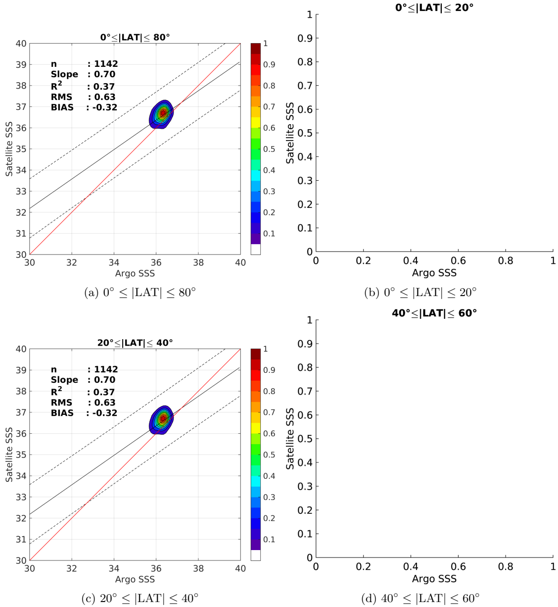
Figure 9: Contour maps of the concentration of Aquarius-L3-JPL-V4-7DAY-RUNNING SSS (y-axis) versus Argo SSS (x-axis) at match-up pairs for different latitude bands. For each plot, the red line shows x=y . The black thin and dashed lines indicate a linear fit through the data cloud and the \pm 95\% confidence levels, respectively. The number match-up pairs n , the slope and R^2 coefficient of the linear fit, the root mean square (RMS) and the mean bias between satellite and in situ data are indicated for each latitude band in each plots.
