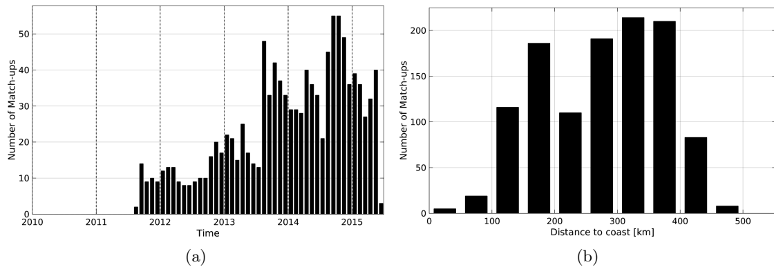
Figure 1: Number of match-ups between Argo and Aquarius-L3-JPL-V4-7DAY-RUNNING SSS as a function of time (a) and as function of the distance to coast (b) over the Mississippi river plume Pi-MEP region and for the full satellite product period.
