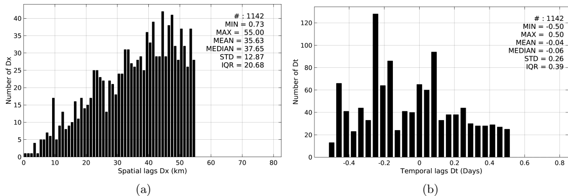
Figure 5: Histograms of the spatial (a) and temporal (b) lags between the time of the Argo measurements and the date of the corresponding Aquarius-L3-JPL-V4-7DAY-RUNNING SSS product.
