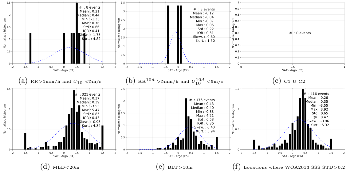
Figure 13: Normalized histogram of \Delta SSS (Aquarius-L3-JPL-V4-7DAY-RUNNING - Argo) for 6 different subdatasets corresponding to: RR > 1mm/h and U_{10} < 5 m/s (a), RR 10d > 5mm/h and U_{10}^{10d} < 5 m/s (b), C1 U C2 (c), MLD < 20m (d), BLT > 10m (e), Locations where WOA2013 SSS STD > 0.2 (f).
