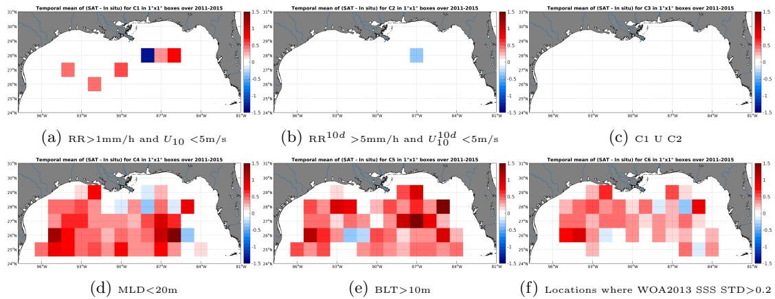
Figure 12: Temporal mean gridded over spatial boxes of size 1^\circ \times 1^\circ of \Delta SSS (Aquarius-L3-JPL-V4-7DAY-RUNNING - Argo) for 6 different subdatasets corresponding to: RR > 1\text{mm/h} and U_{10} < 5\text{m/s} (a), RR^{10d} > 5\text{mm/h} and U_{10}^{10d} < 5\text{m/s} (b), C1 U C2 (c), MLD < 20\text{m} (d), BLT > 10\text{m} (e), Locations where WOA2013 SSS STD > 0.2 (f).
