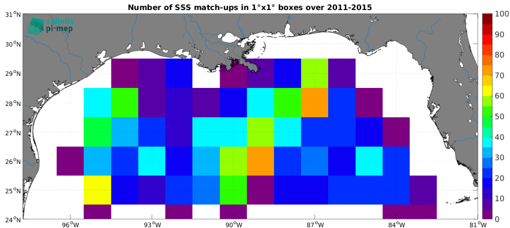
Figure 5: Number of SSS match-ups between Argo SSS and the Aquarius SSS L2-AVERAGED CAP v5 (JPL) SSS product for the Mississippi river plume Pi-MEP region over 1^\circ \times 1^\circ boxes and for the full satellite product period.
