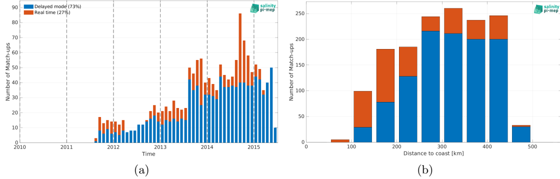
Figure 2: Number of match-ups between Argo and Aquarius SSS L2-AVERAGED CAP v5 (JPL) SSS as a function of time (a) and as function of the distance to coast (b) over the Mississippi river plume Pi-MEP region and for the full satellite product period.
