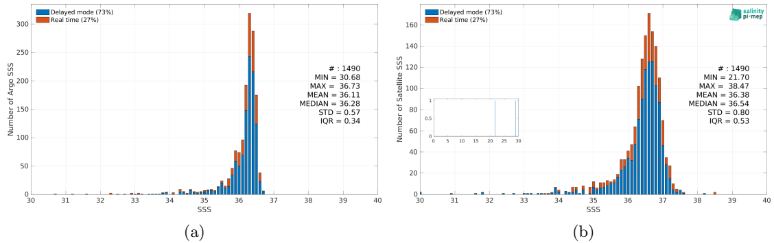
Figure 3: Histograms of SSS from Argo (a) and Aquarius SSS L2-AVERAGED CAP v5 (JPL) (b) considering all match-up pairs per bins of 0.1 over the Mississippi river plume Pi-MEP region and for the full satellite product period.
