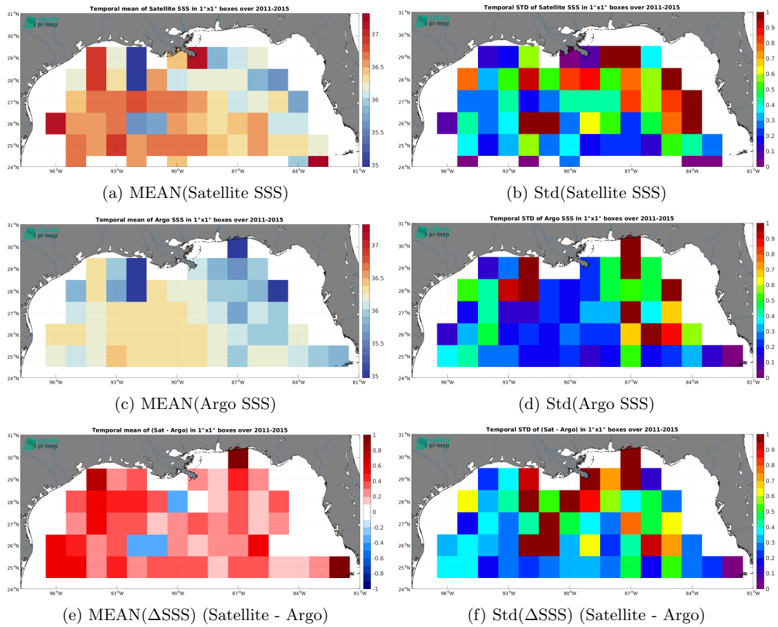
Figure 7: Temporal mean (left) and Std (right) of SSS from Aquarius SSS L2-AVERAGED CAP v5 (JPL) (top), Argo (middle), and of \Delta SSS (Satellite - Argo). Only match-up pairs are used to generate these maps.
