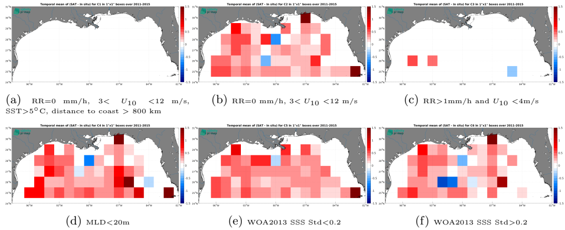
Figure 14: Temporal mean gridded over spatial boxes of size 1^\circ \times 1^\circ of \Delta SSS (Aquarius SSS L2-AVERAGED CAP v5 (JPL) - Argo) for 6 different subdatasets corresponding to:RR=0 mm/h, 3 < U_{10} < 12 m/s, SST>5°C, distance to coast > 800 km (a), RR=0 mm/h, 3 < U_{10} < 12 m/s (b), RR>1mm/h and U_{10} < 4 m/s (c),MLD<20m (d),WOA2013 SSS Std<0.2 (e),WOA2013 SSS Std>0.2 (f).
