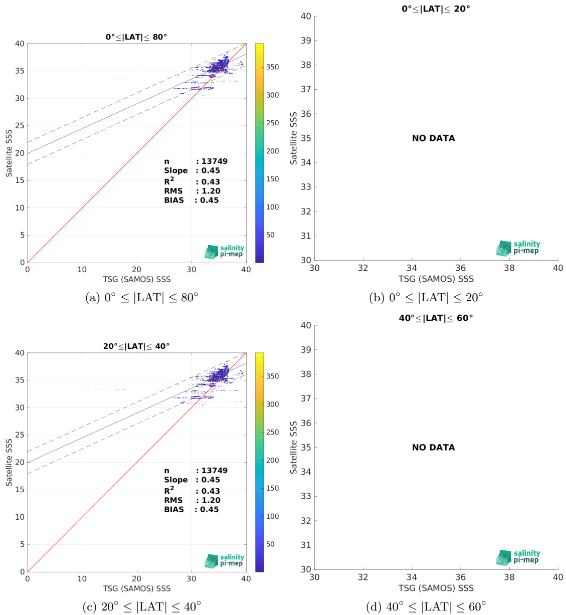
Figure 10: Contour maps of the concentration of Aquarius SSS L2 CAP v5 (JPL) SSS (y-axis) versus TSG (SAMOS) SSS (x-axis) at match-up pairs for different latitude bands. For each plot, the red line shows x=y . The black thin and dashed lines indicate a linear fit through the data cloud and the \pm 95\% confidence levels, respectively. The number match-up pairs n , the slope and R^2 coefficient of the linear fit, the root mean square (RMS) and the mean bias between satellite and in situ data are indicated for each latitude band in each plots.
