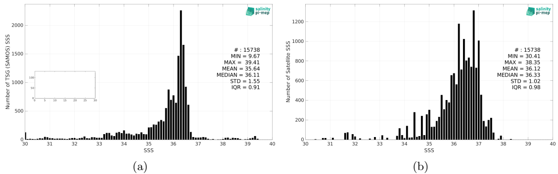
Figure 2: Histograms of SSS from TSG (SAMOS) (a) and Aquarius SSS L2 CAP v5 (JPL) (b) considering all match-up pairs per bins of 0.1 over the Mississippi river plume Pi-MEP region and for the full satellite product period.
