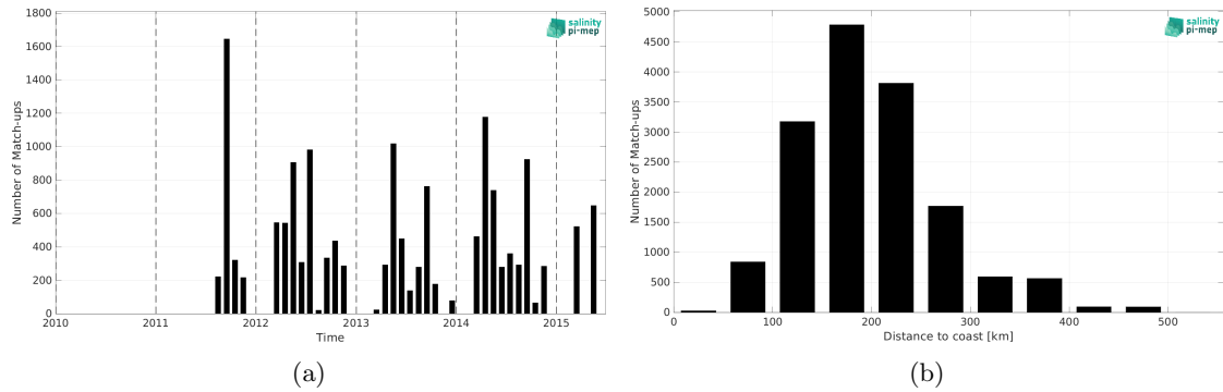
Figure 1: Number of match-ups between TSG (SAMOS) and Aquarius SSS L2 CAP v5 (JPL) SSS as a function of time (a) and as function of the distance to coast (b) over the Mississippi river plume Pi-MEP region and for the full satellite product period.
