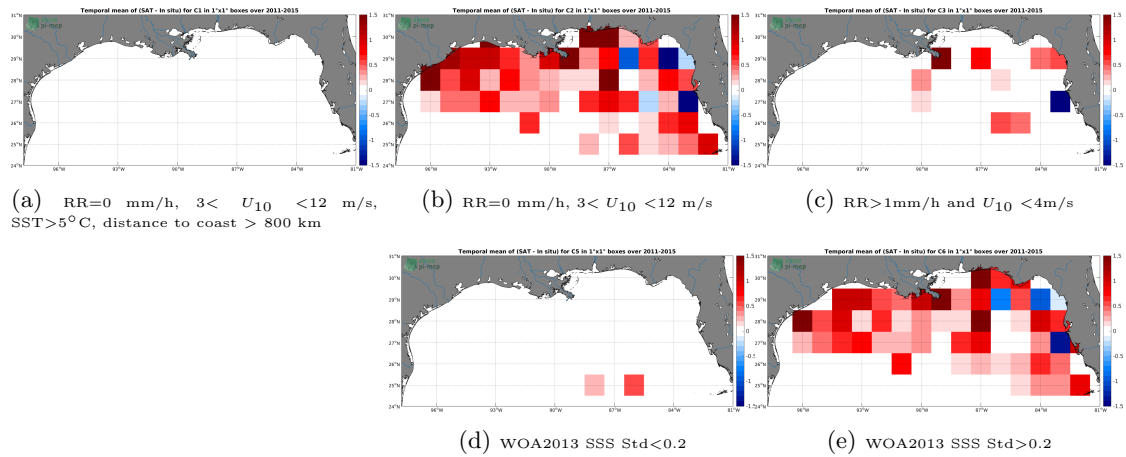
Figure 12: Temporal mean gridded over spatial boxes of size 1^{\circ}\times 1^{\circ} of \Delta\text{SSS} (Aquarius-L2-JPL-V5 - TSG-SAMOS) for 5 different subdatasets corresponding to:RR=0 mm/h, 3 < U_{10} < 12 m/s, SST >5^{\circ}\text{C} , distance to coast > 800 km (a), RR=0 mm/h, 3 < U_{10} < 12 m/s (b), RR >1 mm/h and U_{10} < 4 m/s (c), WOA2013 SSS Std <0.2 (d), WOA2013 SSS Std >0.2 (e).
