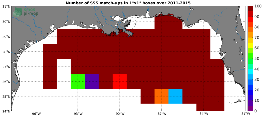
Figure 4: Number of SSS match-ups between TSG-SAMOS SSS and the Aquarius-L2-JPL-V5 SSS product for the Mississippi river plume Pi-MEP region over 1°x1° boxes and for the full satellite product period.
