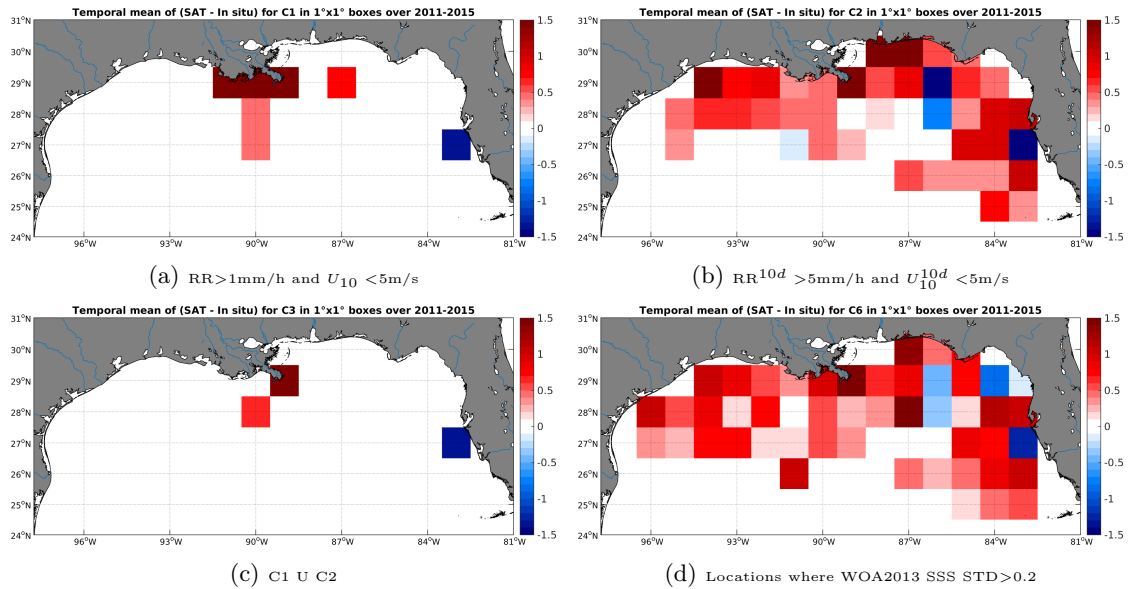
Figure 12: Temporal mean gridded over spatial boxes of size 1^\circ \times 1^\circ of \Delta SSS (AQUARIUS-L2-JPL-V4 - TSG-SAMOS) for 4 different subdatasets corresponding to: RR > 1\text{mm/h} and U_{10} < 5\text{m/s} (a), RR^{10d} > 5\text{mm/h} and U_{10}^{10d} < 5\text{m/s} (b), C1 U C2 (c), Locations where WOA2013 SSS STD > 0.2 (d).
