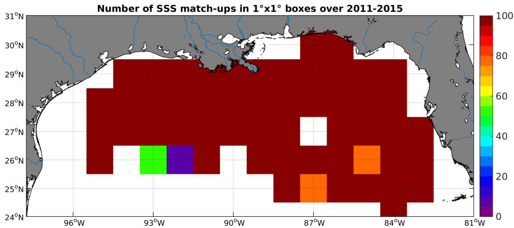
Figure 4: Number of SSS match-ups between TSG-SAMOS SSS and the AQUARIUS-L2-JPL-V4 SSS product for the Mississippi river plume Pi-MEP region over 1^\circ \times 1^\circ boxes and for the full satellite product period.
