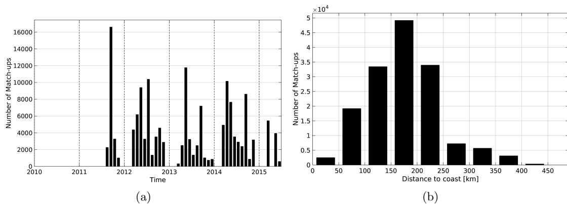
Figure 1: Number of match-ups between TSG-SAMOS and AQUARIUS-L2-JPL-V4 SSS as a function of time (a) and as function of the distance to coast (b) over the Mississippi river plume Pi-MEP region and for the full satellite product period.
