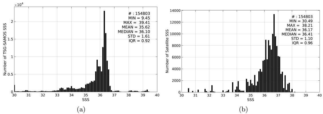
Figure 2: Histograms of SSS from TSG-SAMOS (a) and AQUARIUS-L2-JPL-V4 (b) considering all match-up pairs per bins of 0.1 over the Mississippi river plume Pi-MEP region and for the full satellite product period.
