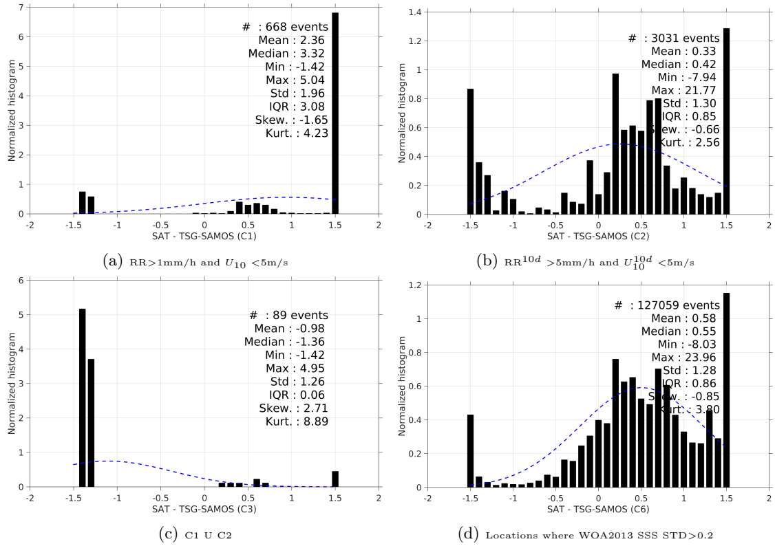
Figure 13: Normalized histogram of \Delta SSS (AQUARIUS-L2-JPL-V4 - TSG-SAMOS) for 6 different subdatasets corresponding to: RR > 1mm/h and U_{10} < 5 m/s (a), RR^{10d} > 5 mm/h and U_{10}^{10d} < 5 m/s (b), C1 U C2 (c), Locations where WOA2013 SSS STD > 0.2 (d).
