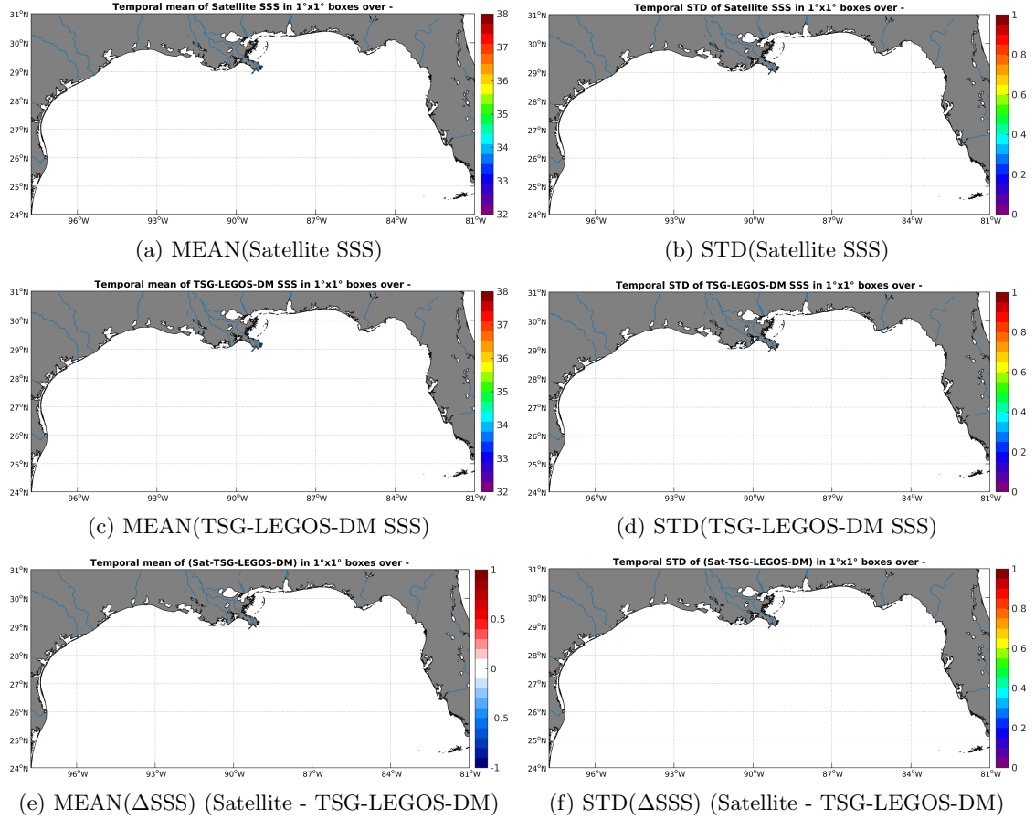
Figure 6: Temporal mean (left) and STD (right) of SSS from AQUARIUS-L2-JPL-V4 (top), TSG-LEGOS-DM (middle), and of \Delta SSS (Satellite - TSG-LEGOS-DM). Only match-up pairs are used to generate these maps.
