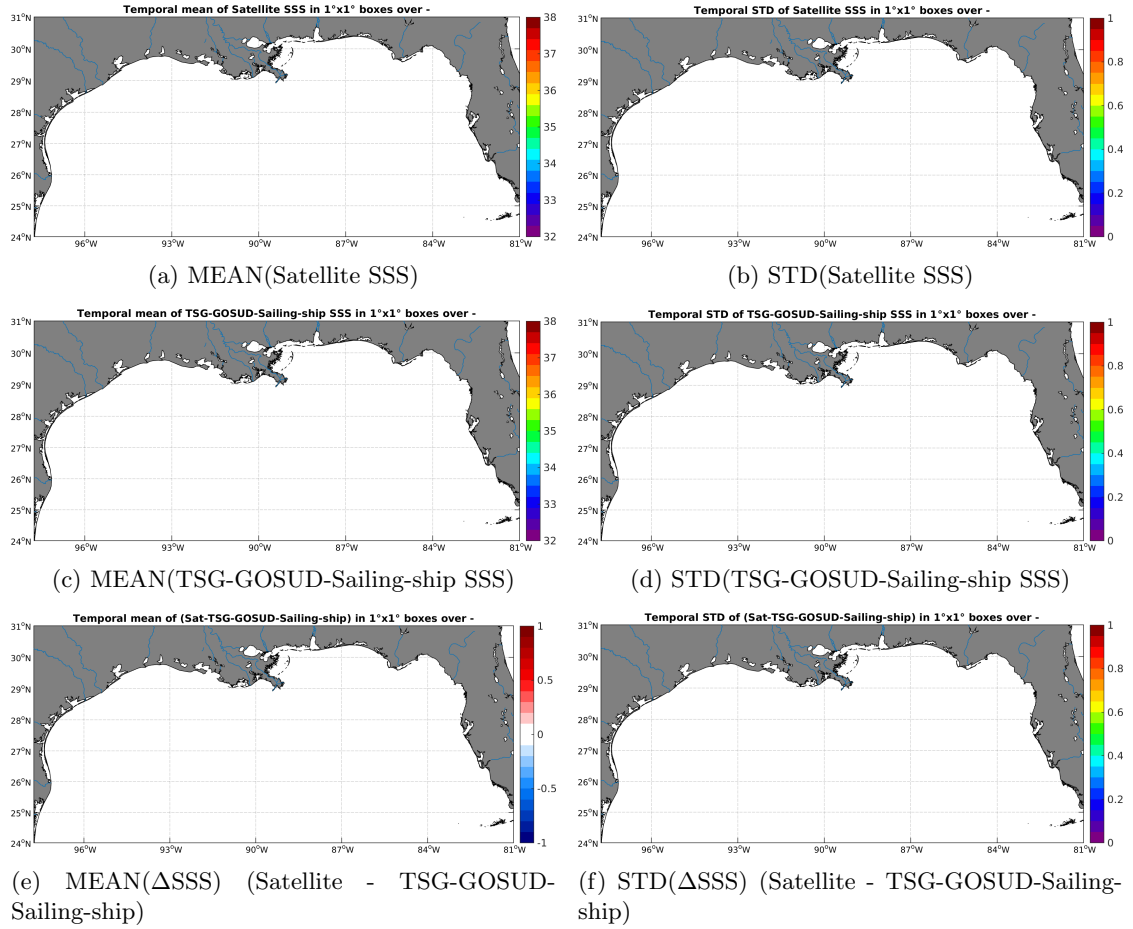
Figure 6: Temporal mean (left) and STD (right) of SSS from AQUARIUS-L2-JPL-V4 (top), TSG-GOSUD-Sailing-ship (middle), and of \Delta SSS (Satellite - TSG-GOSUD-Sailing-ship). Only match-up pairs are used to generate these maps.
