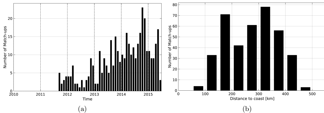
Figure 1: Number of match-ups between Argo and AQUARIUS-L2-JPL-V4 SSS as a function of time (a) and as function of the distance to coast (b) over the Mississippi river plume Pi-MEP region and for the full satellite product period.
