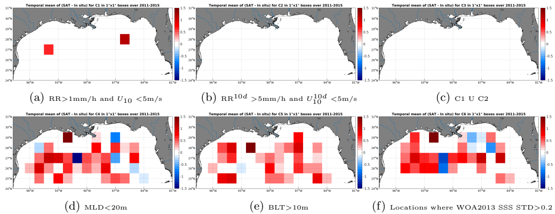
Figure 12: Temporal mean gridded over spatial boxes of size 1^\circ \times 1^\circ of \Delta\text{SSS} (AQUARIUS-L2-JPL-V4 - Argo) for 6 different subdatasets corresponding to: RR > 1\text{mm/h} and U_{10} < 5\text{m/s} (a), RR^{10d} > 5\text{mm/h} and U_{10}^{10d} < 5\text{m/s} (b), C1 U C2 (c), MLD < 20\text{m} (d), BLT > 10\text{m} (e), Locations where WOA2013 SSS STD > 0.2 (f).
