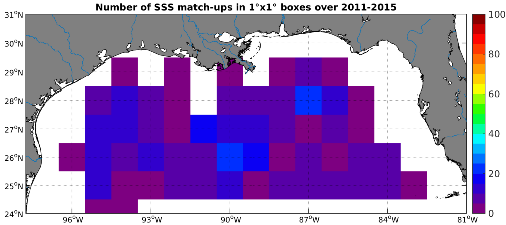
Figure 4: Number of SSS match-ups between Argo SSS and the AQUARIUS-L2-JPL-V4 SSS product for the Mississippi river plume Pi-MEP region over 1^\circ \times 1^\circ boxes and for the full satellite product period.
