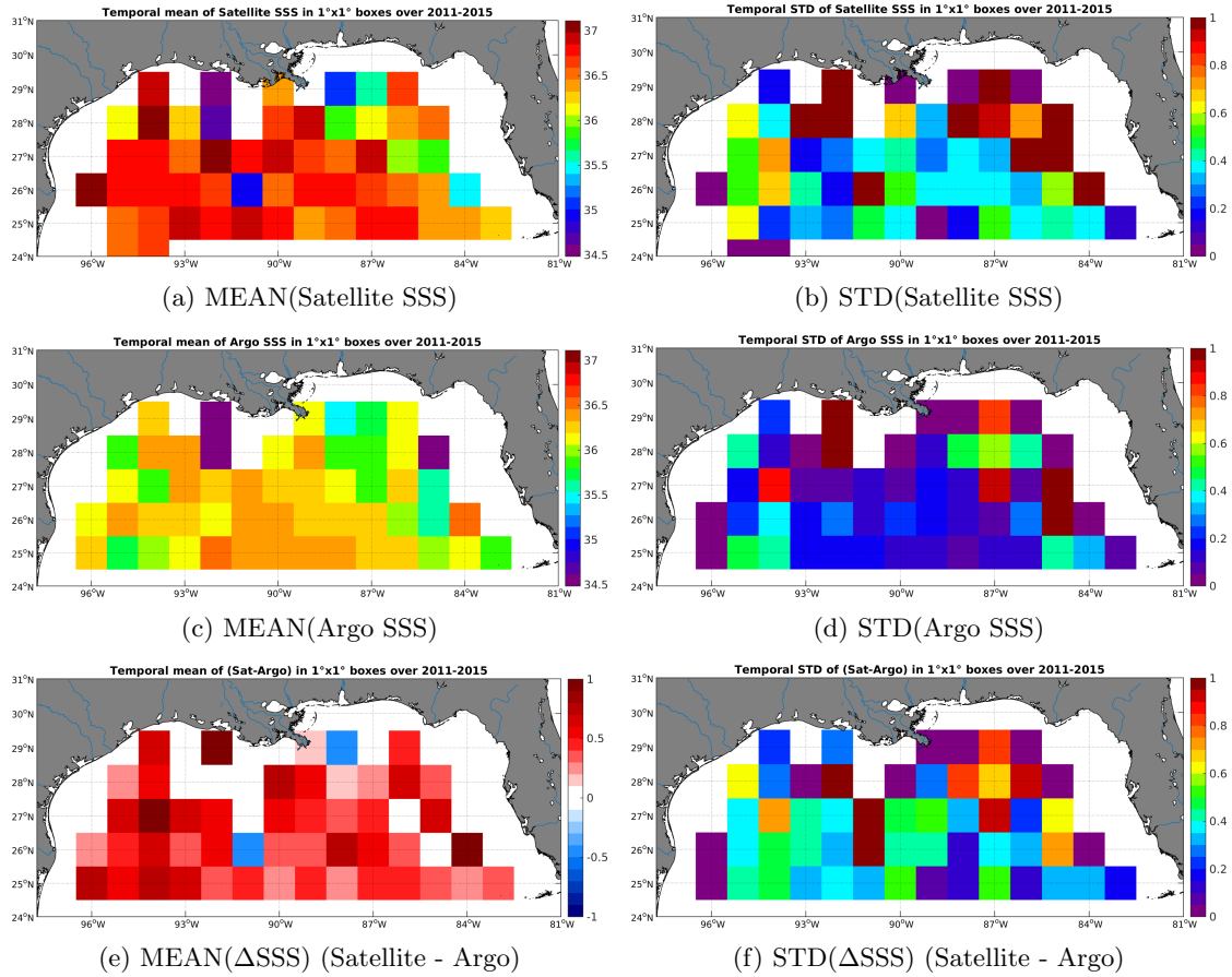
Figure 6: Temporal mean (left) and STD (right) of SSS from AQUARIUS-L2-JPL-V4 (top), Argo (middle), and of \Delta SSS (Satellite - Argo). Only match-up pairs are used to generate these maps.
