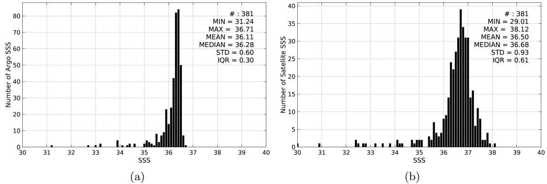
Figure 2: Histograms of SSS from Argo (a) and AQUARIUS-L2-JPL-V4 (b) considering all match-up pairs per bins of 0.1 over the Mississippi river plume Pi-MEP region and for the full satellite product period.
