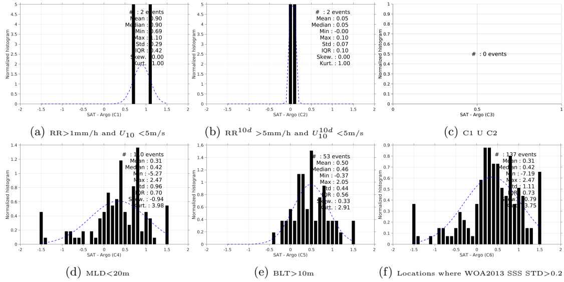
Figure 13: Normalized histogram of \Delta SSS (AQUARIUS-L2-JPL-V4 - Argo) for 6 different sub-datasets corresponding to: RR>1mm/h and U_{10} < 5 m/s (a), RR^{10d} > 5 mm/h and U_{10}^{10d} < 5 m/s (b), C1 U C2 (c),MLD<20m (d),BLT>10m (e),Locations where WOA2013 SSS STD>0.2 (f).
