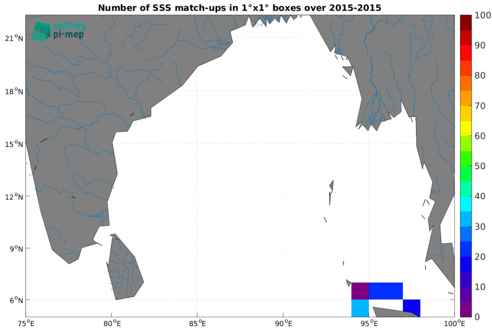
Figure 4: Number of SSS match-ups between TSG (SAMOS) SSS and the SMOS and SMAP SSS L4 OI v1 - 7 Days (LOPS) SSS product for the Ganga and Brahmaputra river plumes Pi-MEP region over 1^{\circ} \times 1^{\circ} boxes and for the full satellite product period.
