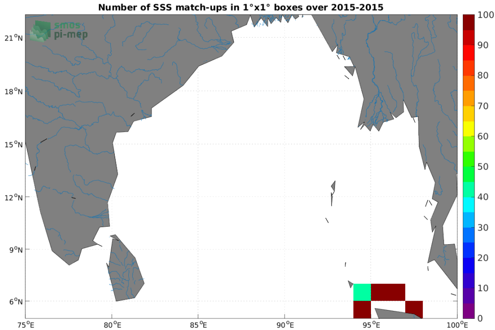
Figure 4: Number of SSS match-ups between TSG (SAMOS) SSS and the SMOS and SMAP SSS L4 OI v1 - 7 Days (LOPS) SSS product for the Ganga and Brahmaputra river plumes Pi-MEP region over 1°x1° boxes and for the full satellite product period.
