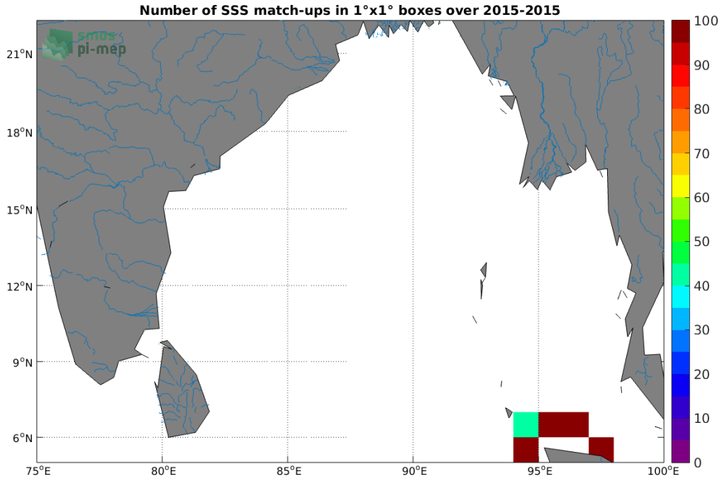
Figure 4: Number of SSS match-ups between TSG (SAMOS) SSS and the SMOS and SMAP SSS L4 OI v1 - 7 Days (LOPS) SSS product for the Ganga and Brahmaputra river plumes Pi-MEP region over 1°×1° boxes and for the full satellite product period.
