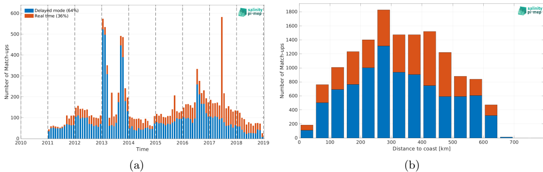
Figure 1: Number of match-ups between Argo and SMOS and SMAP SSS L4 OI v1 - 7 Days (LOPS) SSS as a function of time (a) and as function of the distance to coast (b) over the Ganga and Brahmaputra river plumes Pi-MEP region and for the full satellite product period.
