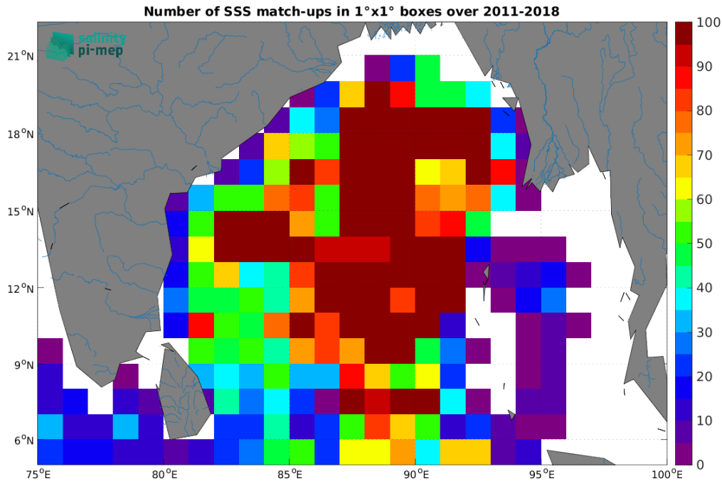
Figure 4: Number of SSS match-ups between Argo SSS and the SMOS and SMAP SSS L4 OI v1 - 7 Days (LOPS) SSS product for the Ganga and Brahmaputra river plumes Pi-MEP region over 1^\circ \times 1^\circ boxes and for the full satellite product period.
