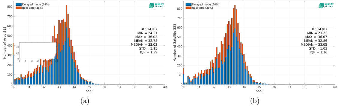
Figure 2: Histograms of SSS from Argo (a) and SMOS and SMAP SSS L4 OI v1 - 7 Days (LOPS) (b) considering all match-up pairs per bins of 0.1 over the Ganga and Brahmaputra river plumes Pi-MEP region and for the full satellite product period.
