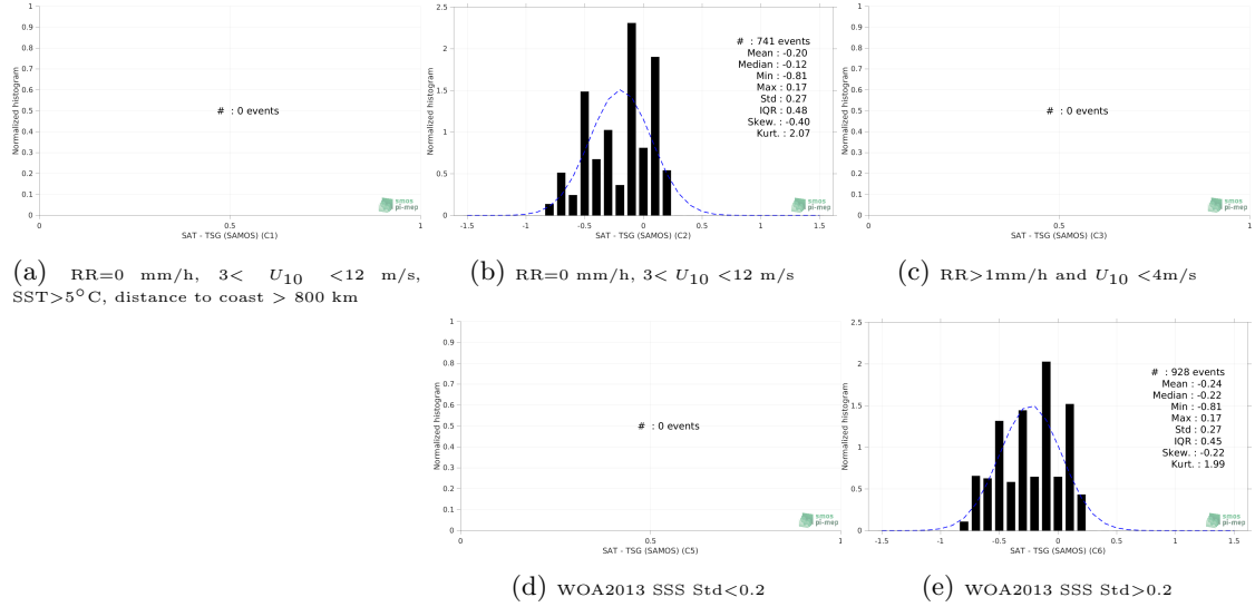
Figure 13: Normalized histogram of \Delta SSS (SMOS SSS L4 v1 - Weekly (CMEMS-CNR) - TSG (SAMOS)) for 5 different subdatasets corresponding to: RR=0 mm/h, 3 < U_{10} < 12 m/s, SST>5°C, distance to coast > 800 km (a), RR=0 mm/h, 3 < U_{10} < 12 m/s (b), RR>1mm/h and U_{10} < 4 m/s (c), WOA2013 SSS Std<0.2 (d), WOA2013 SSS Std>0.2 (e).
