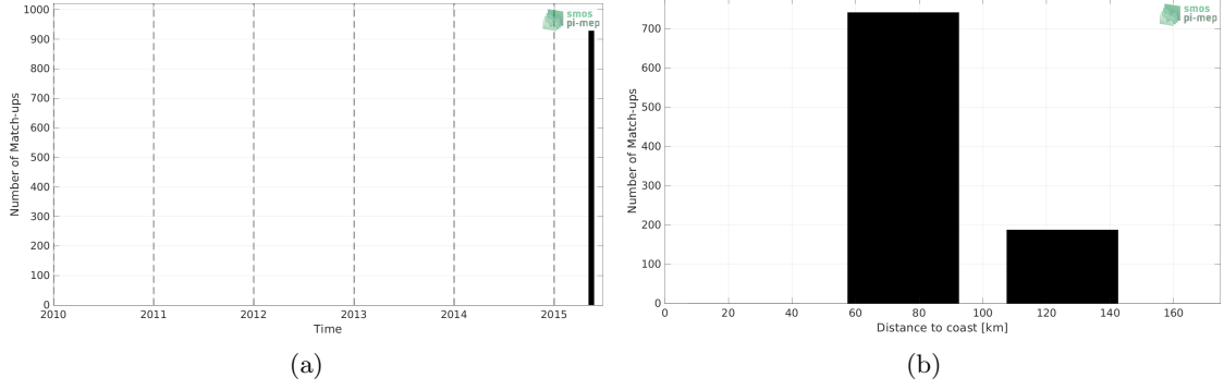
Figure 1: Number of match-ups between TSG (SAMOS) and SMOS SSS L4 v1 - Weekly (CMEMS-CNR) SSS as a function of time (a) and as function of the distance to coast (b) over the Ganga and Brahmaputra river plumes Pi-MEP region and for the full satellite product period.
