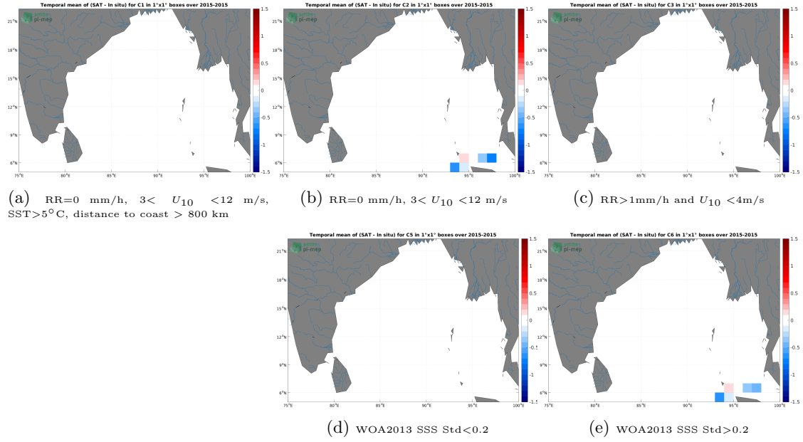
Figure 12: Temporal mean gridded over spatial boxes of size 1^\circ \times 1^\circ of \Delta SSS (SMOS SSS L4 v1 - Weekly (CMEMS-CNR) - TSG (SAMOS)) for 5 different subdatasets corresponding to: RR=0 mm/h, 3 < U_{10} < 12 m/s, SST > 5^\circ C , distance to coast > 800 km (a), RR=0 mm/h, 3 < U_{10} < 12 m/s (b), RR > 1 mm/h and U_{10} < 4 m/s (c), WOA2013 SSS Std < 0.2 (d), WOA2013 SSS Std > 0.2 (e).
