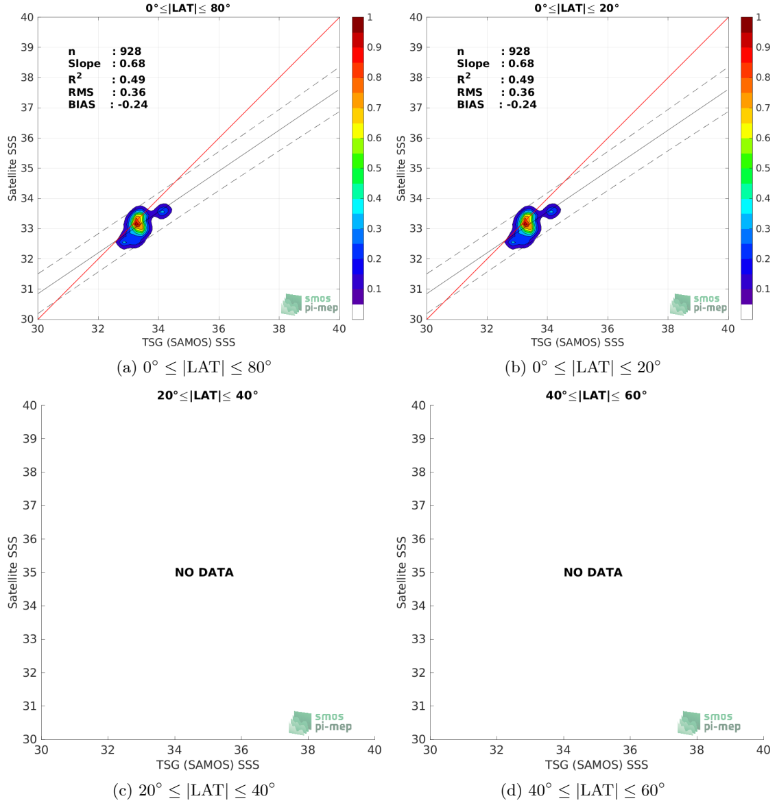
Figure 9: Contour maps of the concentration of SMOS SSS L4 v1 - Weekly (CMEMS-CNR) SSS (y-axis) versus TSG (SAMOS) SSS (x-axis) at match-up pairs for different latitude bands. For each plot, the red line shows x=y . The black thin and dashed lines indicate a linear fit through the data cloud and the \pm 95\% confidence levels, respectively. The number match-up pairs n , the slope and R^2 coefficient of the linear fit, the root mean square (RMS) and the mean bias between satellite and in situ data are indicated for each latitude band in each plots.
