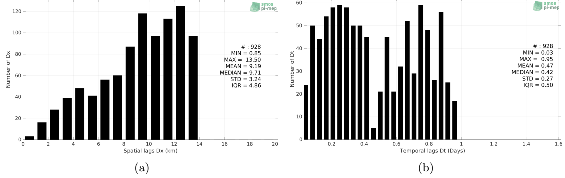
Figure 5: Histograms of the spatial (a) and temporal (b) lags between the location/time of the TSG (SAMOS) measurement and the date of the corresponding SMOS SSS L4 v1 - Weekly (CMEMS-CNR) SSS pixel.
