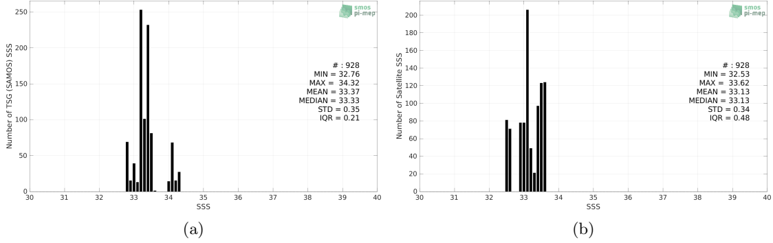
Figure 2: Histograms of SSS from TSG (SAMOS) (a) and SMOS SSS L4 v1 - Weekly (CMEMS-CNR) (b) considering all match-up pairs per bins of 0.1 over the Ganga and Brahmaputra river plumes Pi-MEP region and for the full satellite product period.
