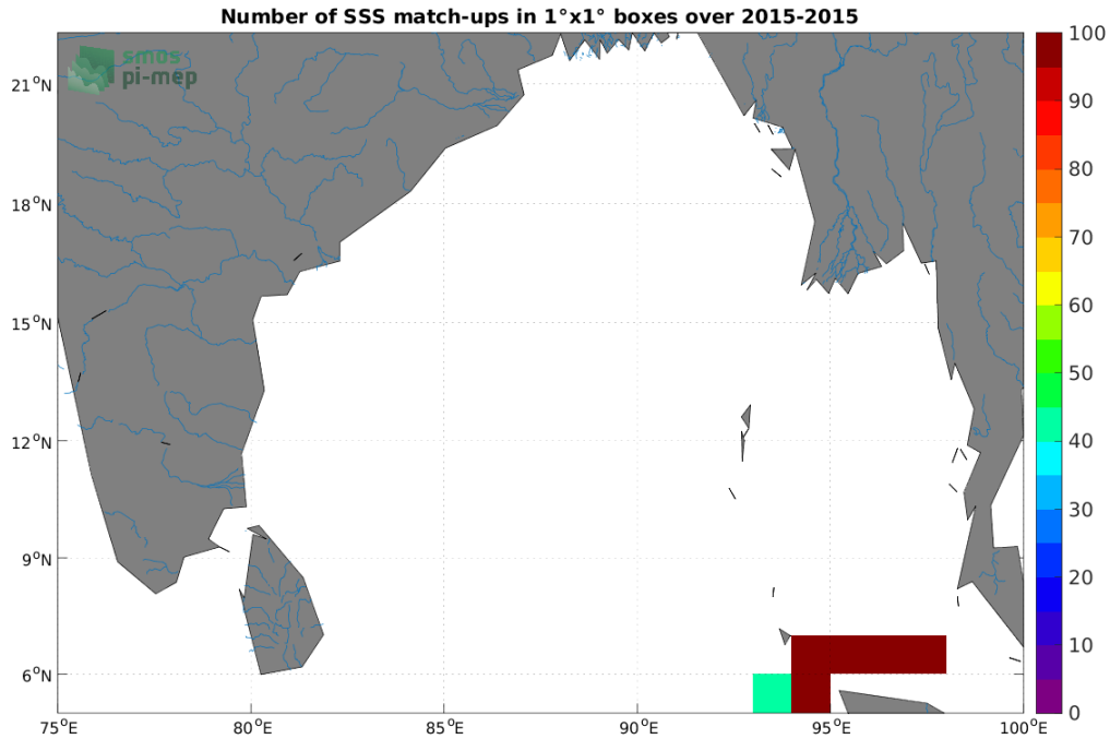
Figure 4: Number of SSS match-ups between TSG (SAMOS) SSS and the SMOS SSS L4 v1 - Weekly (CMEMS-CNR) SSS product for the Ganga and Brahmaputra river plumes Pi-MEP region over 1^\circ \times 1^\circ boxes and for the full satellite product period.
