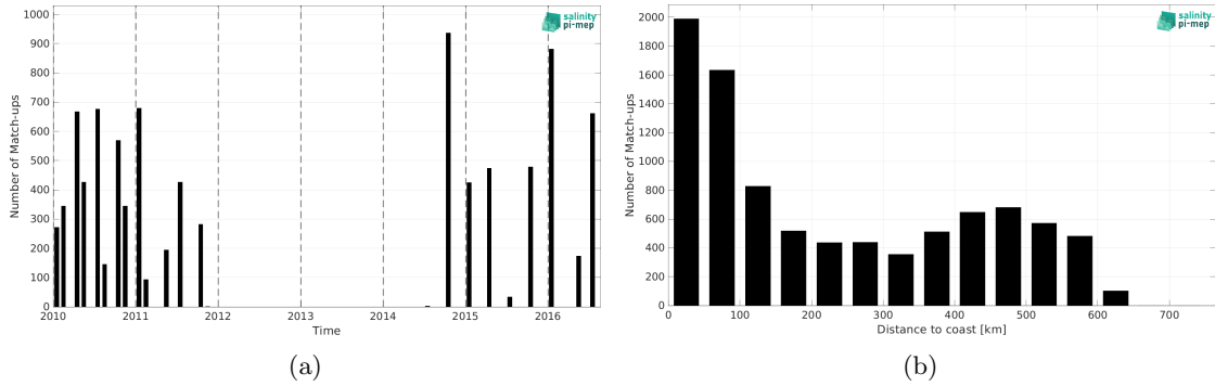
Figure 1: Number of match-ups between TSG (LEGOS-DM) and SMOS SSS L4 v1 - Weekly (CMEMS-CNR) SSS as a function of time (a) and as function of the distance to coast (b) over the Ganga and Brahmaputra river plumes Pi-MEP region and for the full satellite product period.
