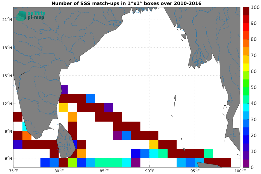
Figure 4: Number of SSS match-ups between TSG (LEGOS-DM) SSS and the SMOS SSS L4 v1 - Weekly (CMEMS-CNR) SSS product for the Ganga and Brahmaputra river plumes Pi-MEP region over 1^\circ \times 1^\circ boxes and for the full satellite product period.
