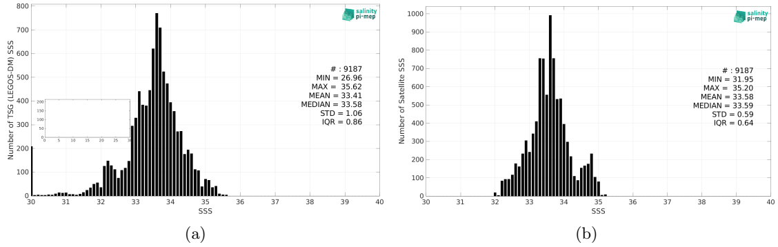
Figure 2: Histograms of SSS from TSG (LEGOS-DM) (a) and SMOS SSS L4 v1 - Weekly (CMEMS-CNR) (b) considering all match-up pairs per bins of 0.1 over the Ganga and Brahmaputra river plumes Pi-MEP region and for the full satellite product period.
