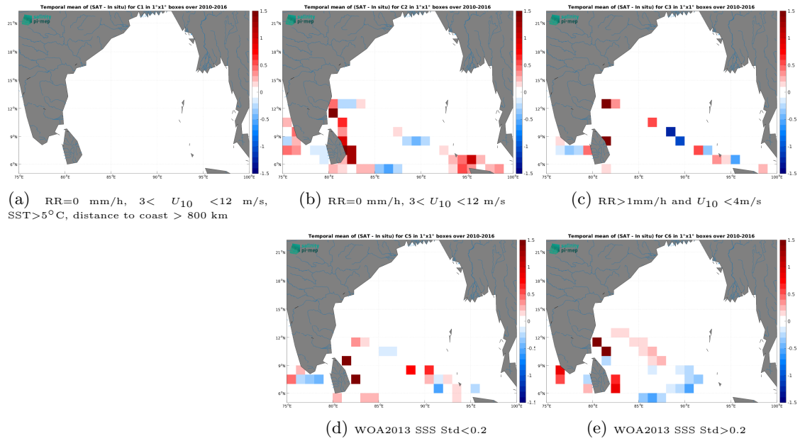
Figure 12: Temporal mean gridded over spatial boxes of size 1^\circ \times 1^\circ of \Delta SSS (SMOS SSS L4 v1 - Weekly (CMEMS-CNR) - TSG (LEGOS-DM)) for 5 different subdatasets corresponding to:RR=0 mm/h, 3 < U_{10} < 12 m/s, SST >5^\circ C, distance to coast > 800 km (a), RR=0 mm/h, 3 < U_{10} < 12 m/s (b), RR >1 mm/h and U_{10} < 4 m/s (c), WOA2013 SSS Std <0.2 (d), WOA2013 SSS Std >0.2 (e).
