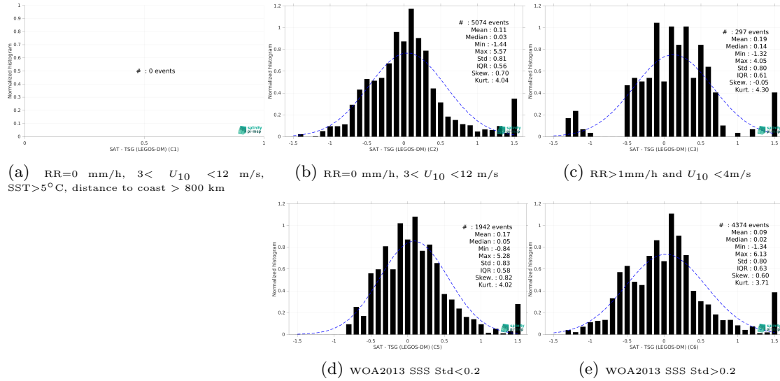
Figure 13: Normalized histogram of \Delta\text{SSS} (SMOS SSS L4 v1 - Weekly (CMEMS-CNR) - TSG (LEGOS-DM)) for 5 different subdatasets corresponding to: RR=0 mm/h, 3 < U_{10} < 12 m/s, SST > 5^\circ\text{C} , distance to coast > 800 km (a), RR=0 mm/h, 3 < U_{10} < 12 m/s (b), RR > 1 mm/h and U_{10} < 4 m/s (c), WOA2013 SSS Std < 0.2 (d), WOA2013 SSS Std > 0.2 (e).
