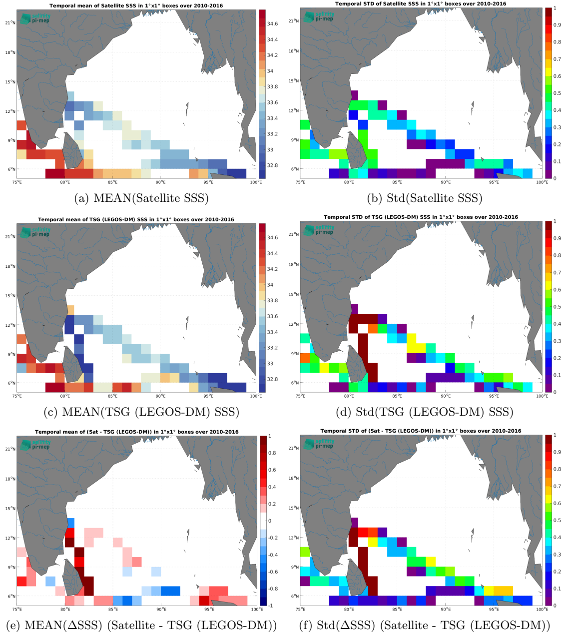
Figure 6: Temporal mean (left) and Std (right) of SSS from SMOS SSS L4 v1 - Weekly (CMEMS-CNR) (top), TSG (LEGOS-DM) (middle), and of \Delta SSS (Satellite - TSG (LEGOS-DM)). Only match-up pairs are used to generate these maps.
