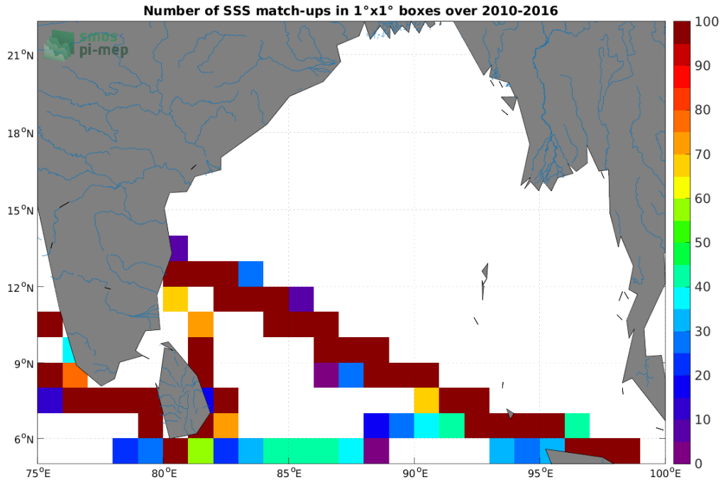
Figure 4: Number of SSS match-ups between TSG (LEGOS-DM) SSS and the SMOS SSS L4 v1 - Weekly (CMEMS-CNR) SSS product for the Ganga and Brahmaputra river plumes Pi-MEP region over 1°×1° boxes and for the full satellite product period.
