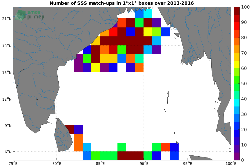
Figure 3: Number of SSS match-ups between Surface drifters SSS and the SMOS SSS L4 v1 - Weekly (CMEMS-CNR) SSS product for the Ganga and Brahmaputra river plumes Pi-MEP region over 1°x1° boxes and for the full satellite product period.
