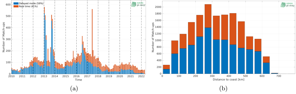
Figure 1: Number of match-ups between Argo and SMOS SSS L4 v1 - Weekly (CMEMS-CNR) SSS as a function of time (a) and as function of the distance to coast (b) over the Ganga and Brahmaputra river plumes Pi-MEP region and for the full satellite product period.
