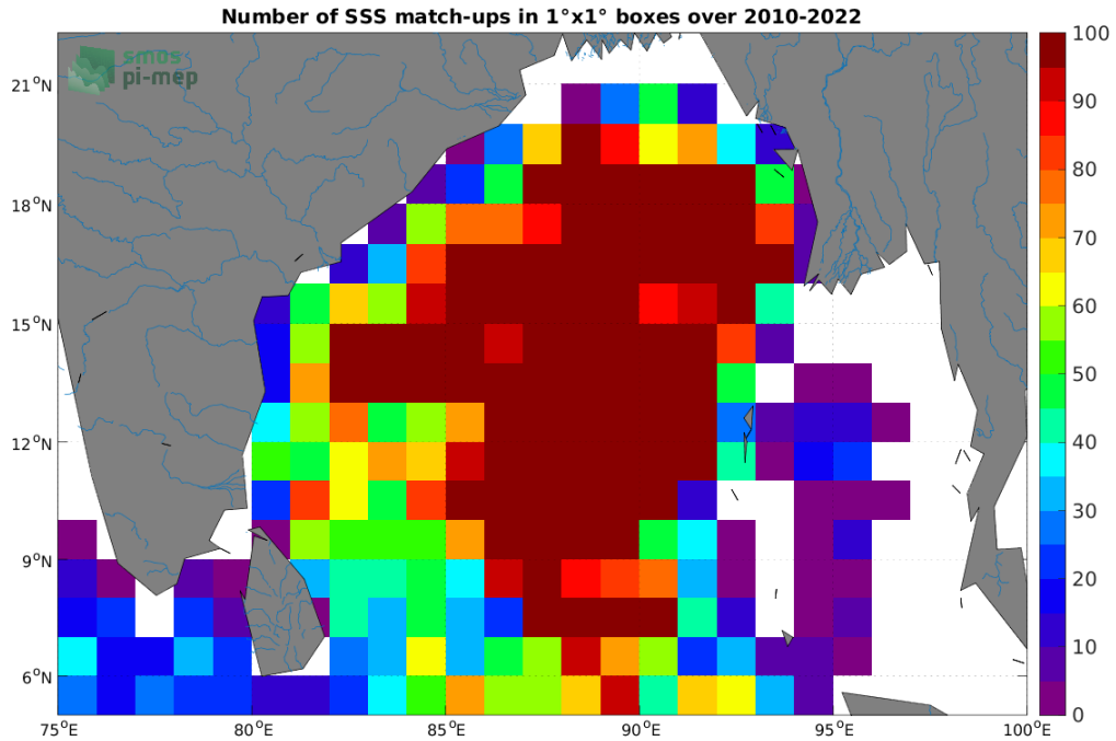
Figure 4: Number of SSS match-ups between Argo SSS and the SMOS SSS L4 v1 - Weekly (CMEMS-CNR) SSS product for the Ganga and Brahmaputra river plumes Pi-MEP region over 1^\circ \times 1^\circ boxes and for the full satellite product period.
