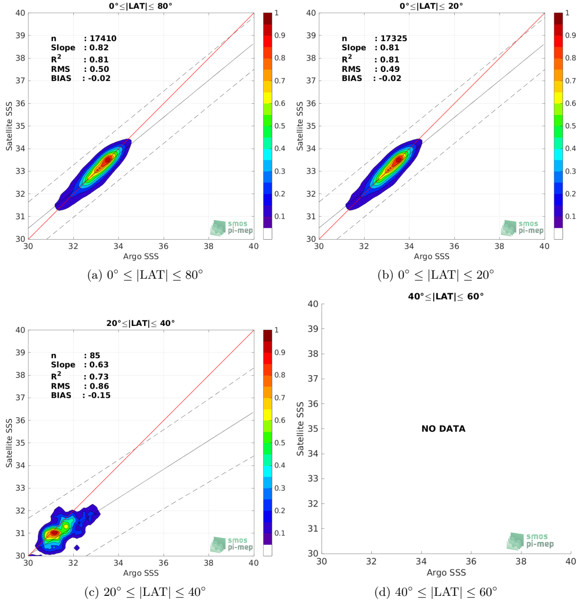
Figure 9: Contour maps of the concentration of SMOS SSS L4 v1 - Weekly (CMEMS-CNR) SSS (y-axis) versus Argo SSS (x-axis) at match-up pairs for different latitude bands. For each plot, the red line shows x=y . The black thin and dashed lines indicate a linear fit through the data cloud and the \pm 95\% confidence levels, respectively. The number match-up pairs n , the slope and R^2 coefficient of the linear fit, the root mean square (RMS) and the mean bias between satellite and in situ data are indicated for each latitude band in each plots.
