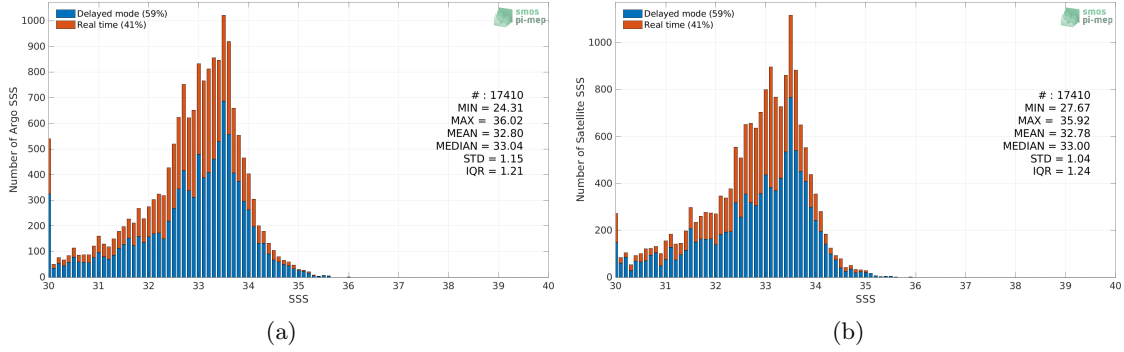
Figure 2: Histograms of SSS from Argo (a) and SMOS SSS L4 v1 - Weekly (CMEMS-CNR) (b) considering all match-up pairs per bins of 0.1 over the Ganga and Brahmaputra river plumes Pi-MEP region and for the full satellite product period.
