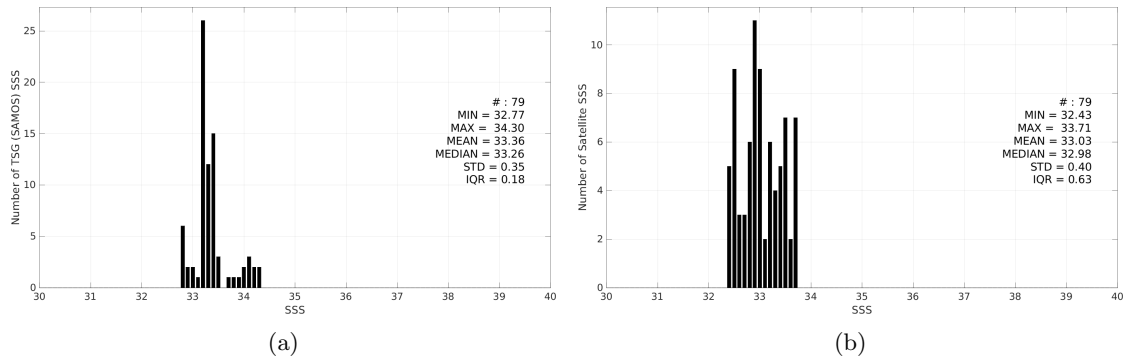
Figure 3: Histograms of SSS from TSG (SAMOS) (a) and SMOS SSS L4 v1 - Monthly (CMEMS-CNR) (b) considering all match-up pairs per bins of 0.1 over the Ganga and Brahmaputra river plumes Pi-MEP region and for the full satellite product period.
