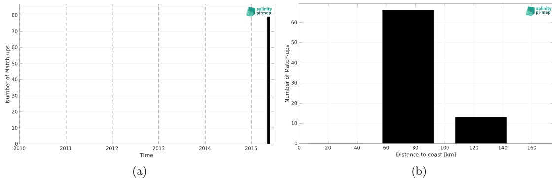
Figure 2: Number of match-ups between TSG (SAMOS) and SMOS SSS L4 v1 - Monthly (CMEMS-CNR) SSS as a function of time (a) and as function of the distance to coast (b) over the Ganga and Brahmaputra river plumes Pi-MEP region and for the full satellite product period.
