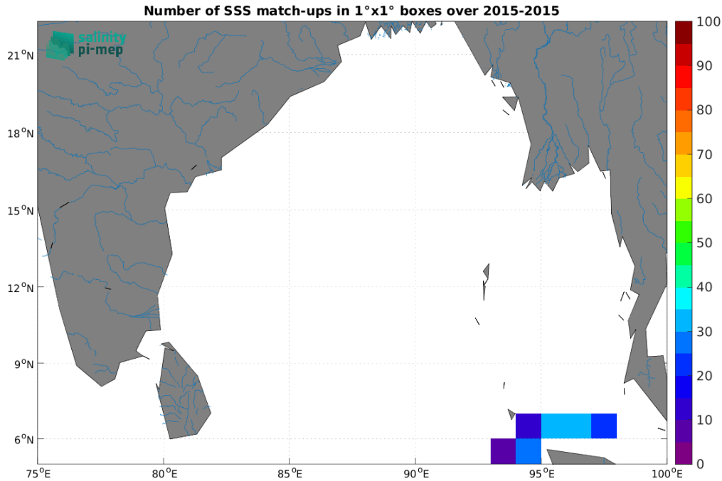
Figure 4: Number of SSS match-ups between TSG (SAMOS) SSS and the SMOS SSS L4 v1 - Monthly (CMEMS-CNR) SSS product for the Ganga and Brahmaputra river plumes Pi-MEP region over 1^\circ \times 1^\circ boxes and for the full satellite product period.
